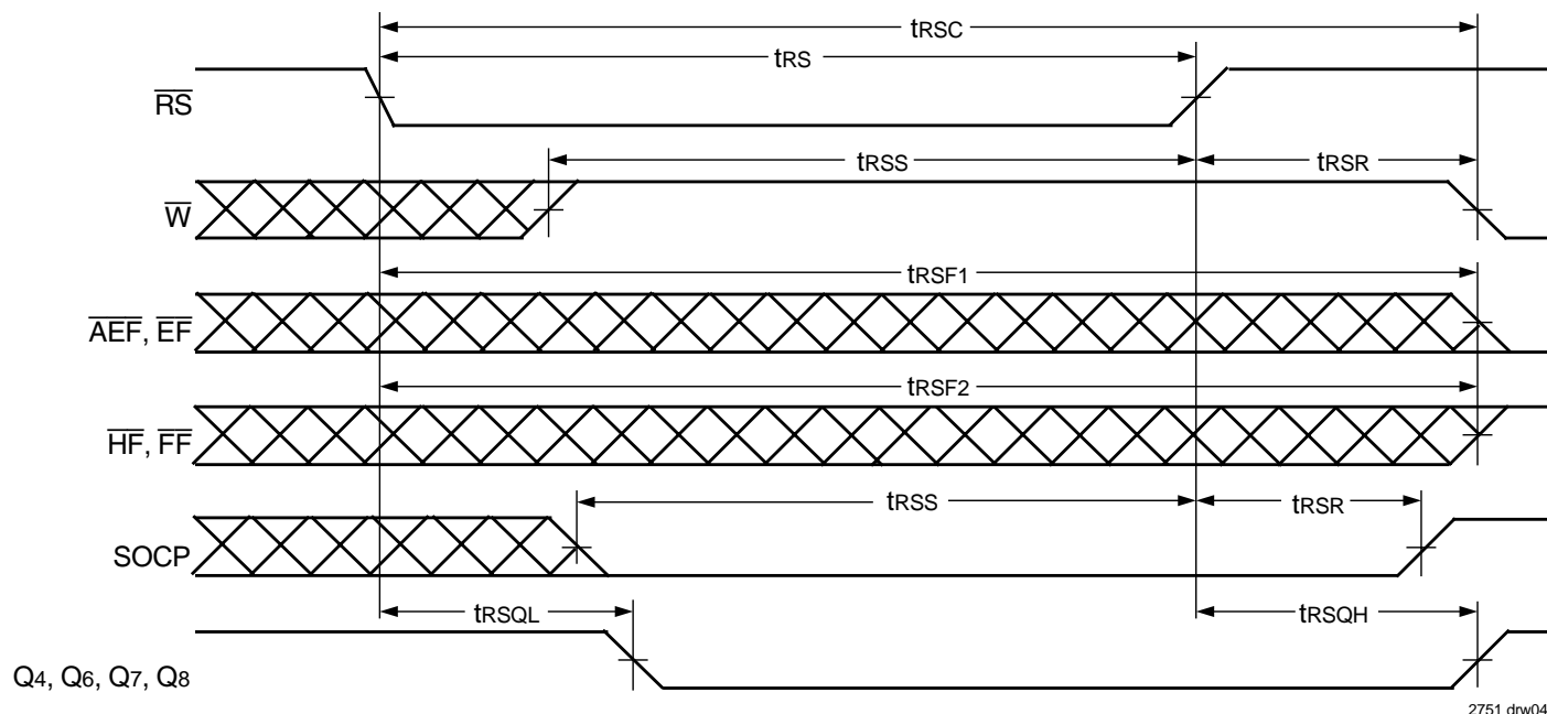
Figure 1. Reset
