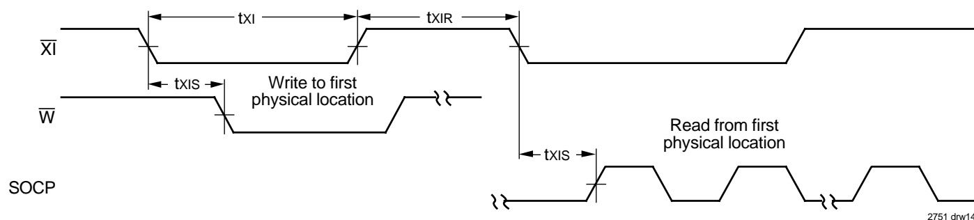
Figure 11. Expansion-In
