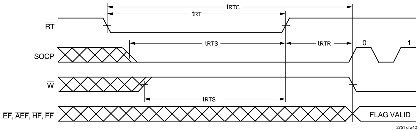
Figure 9. Retransmit
