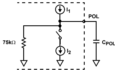
FIGURE 7. REVERSAL TIMING CONTROL
