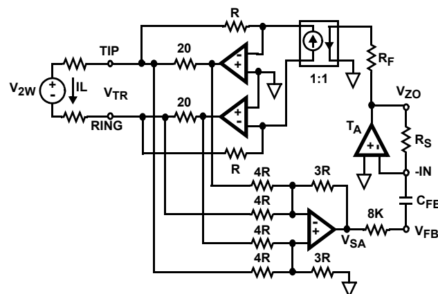
FIGURE 11. IMPEDANCE SYNTHESIS
