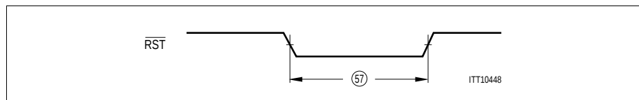
Figure 106 Reset Timing
