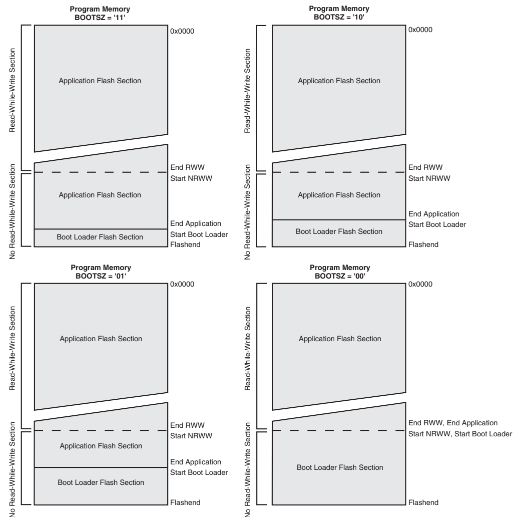
Figure 28-2. Memory Sections
