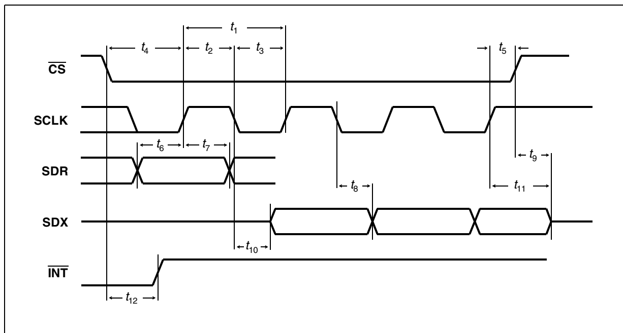
Figure 72 SCI Interface
