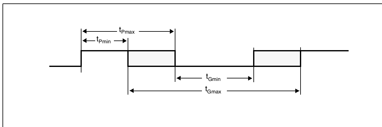
Figure 35 Call Progress Tone Detector- Cooked Mode
