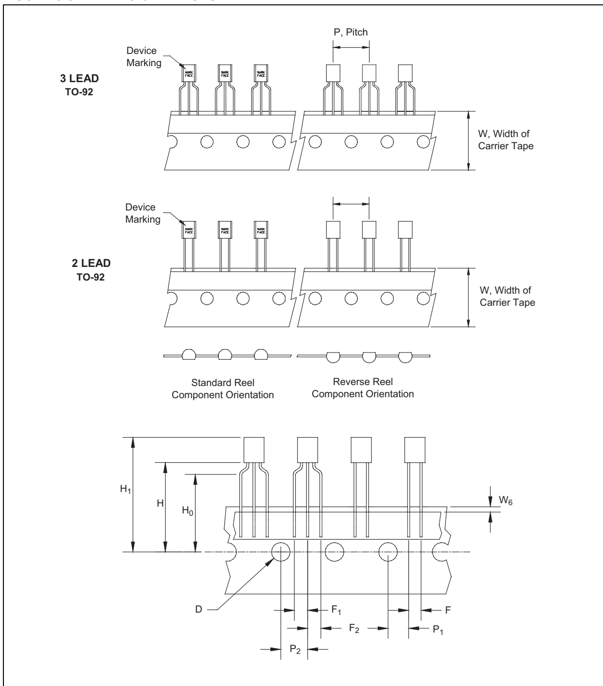
FIGURE 5-3: TO-92 DEVICES
