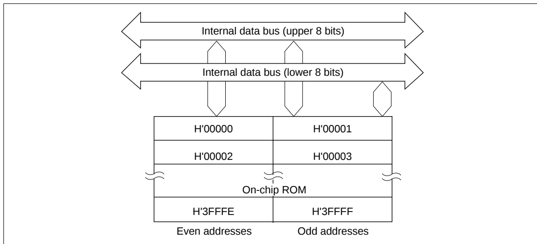
Figure 15-20 Block Diagram of ROM (H8/3022)
