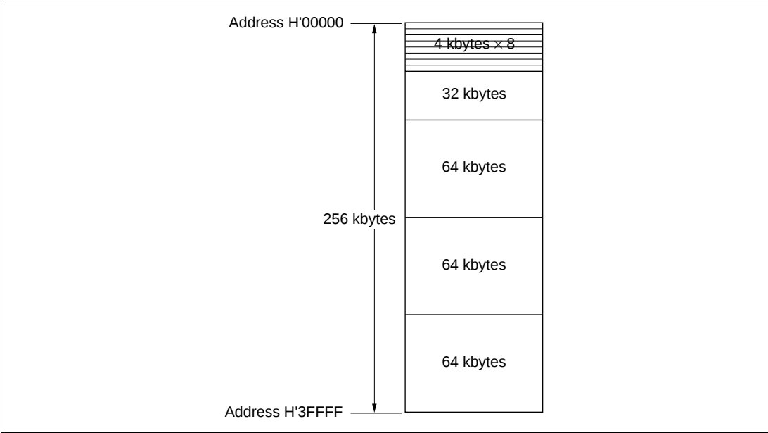
Figure 15-5 Block Configuration
