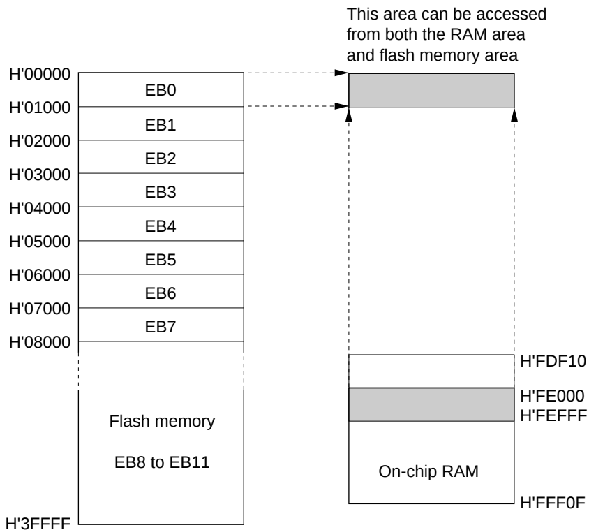
Figure 15-15 Example of RAM Overlap Operation
