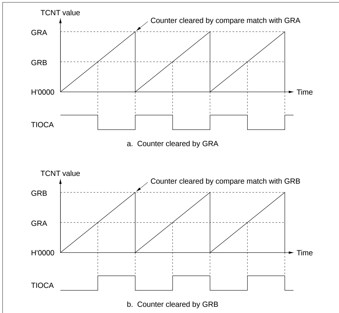
Figure 8-29 PWM Mode (Example 1)
