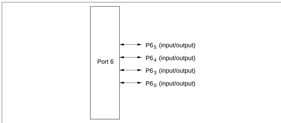
Figure 7-18 Pin Functions in Mode 7 (Port 6)
