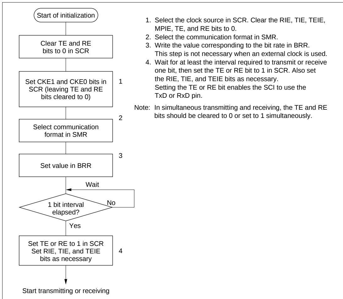
Figure 11-15 Sample Flowchart for SCI Initialization
