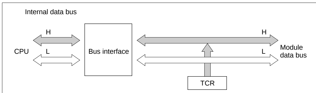
Figure 8-13 TCR Access (CPU Reads TCR)
