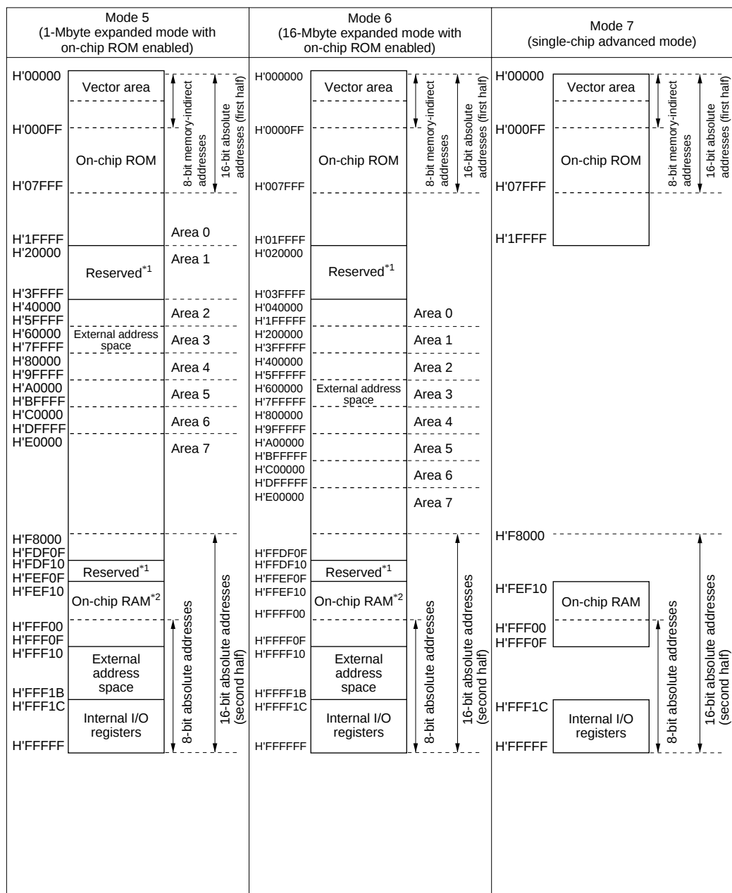
Figure 3-3 H8/3020 Memory Map in Each Operating Mode (2)
