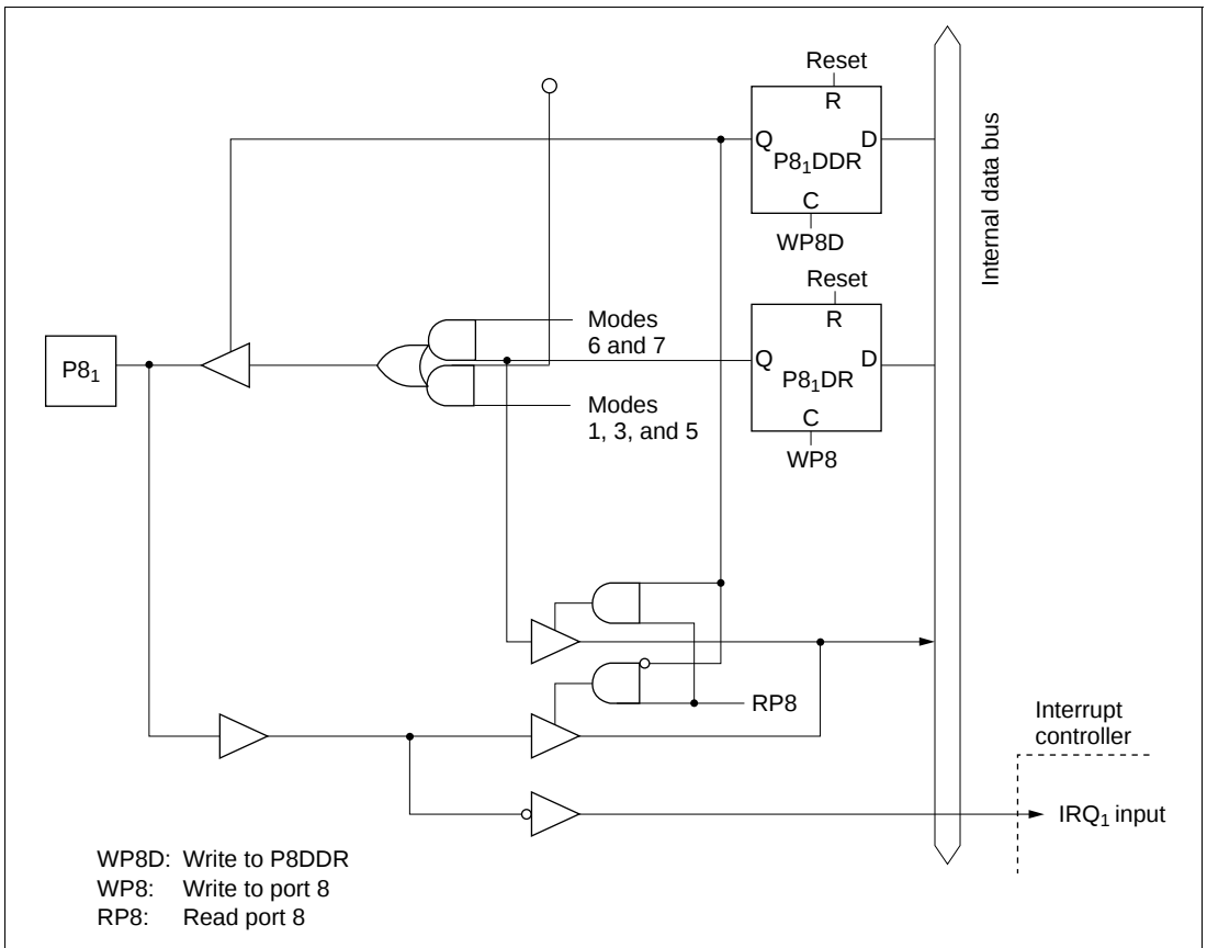
Figure C-7 (b) Port 8 Block Diagram (Pin P8 1 )
