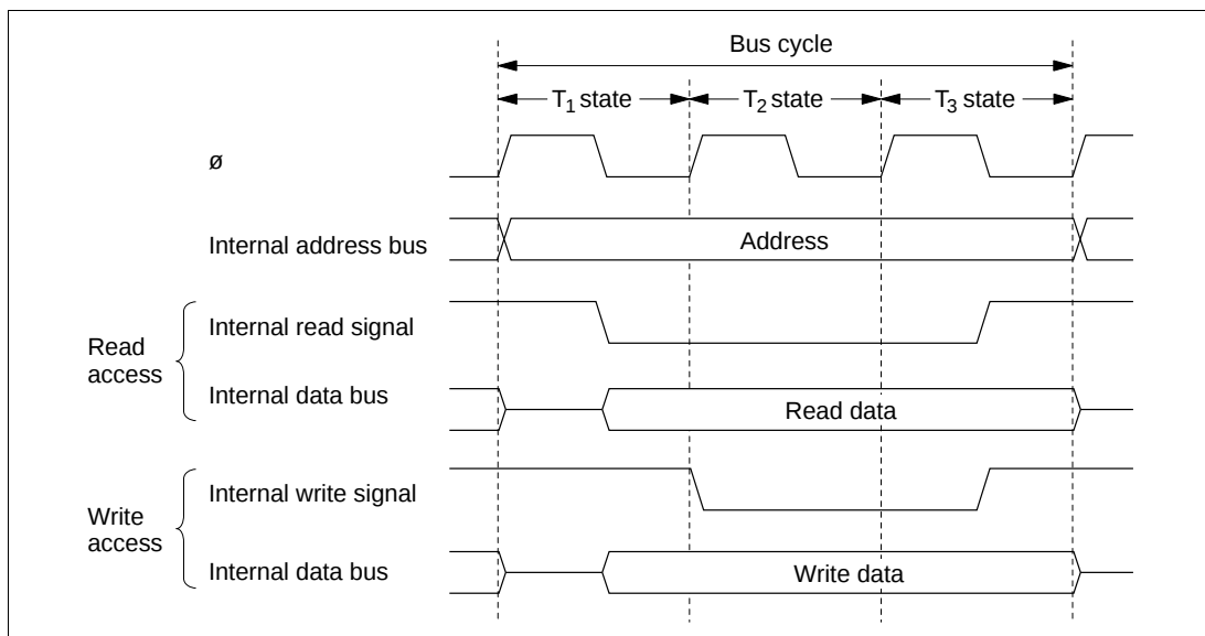
Figure 2-17 Access Cycle for On-Chip Supporting Modules
