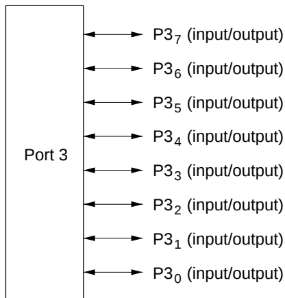
Figure 7-11 Pin Functions in Mode 7 (Port 3)
