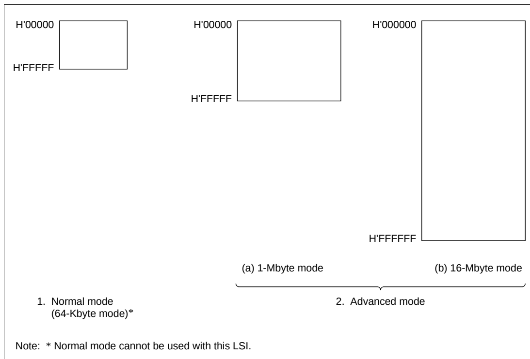
Figure 2-2 Memory Map
