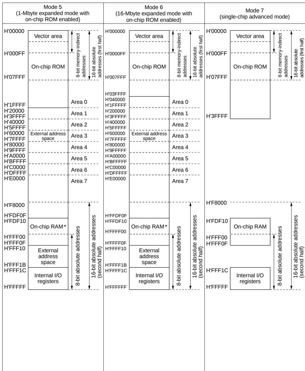
Figure 3-1 H8/3022 Memory Map in Each Operating Mode (2)
