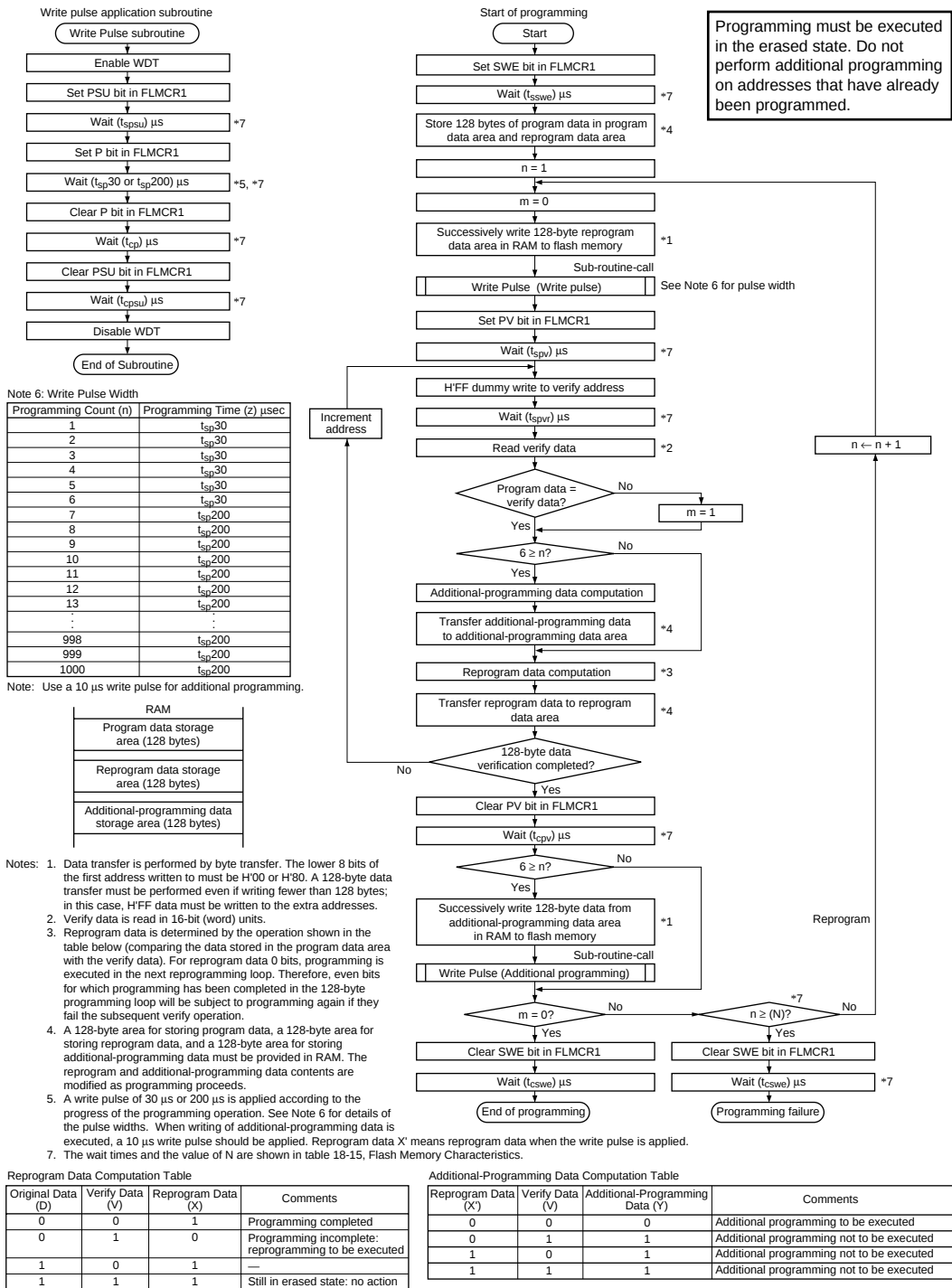
Figure 15-11 H8/3022F Program/Program-Verify Flowchart
