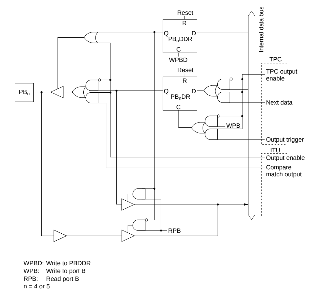
Figure C-10 (b) Port B Block Diagram (Pins PB 4 and PB 5 )
