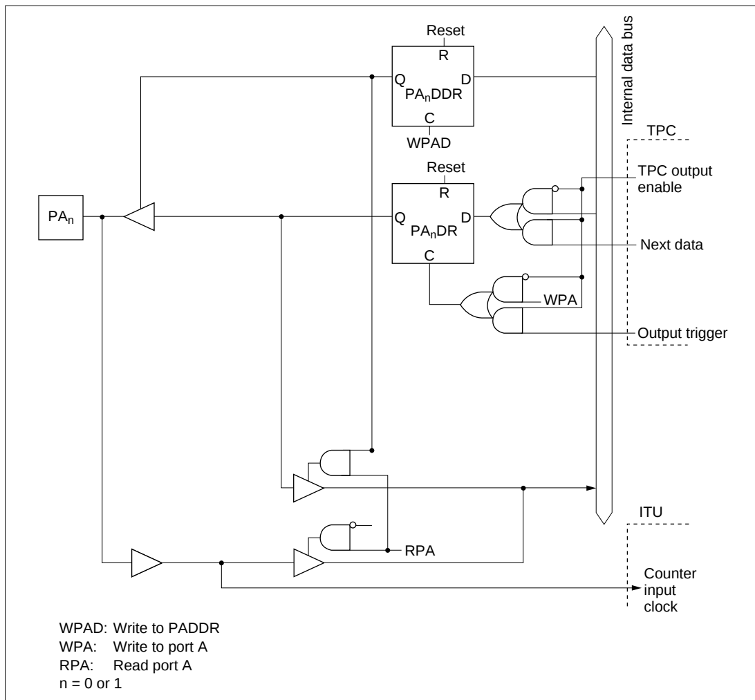
Figure C-9 (a) Port A Block Diagram (Pins PA 0 and PA 1 )
