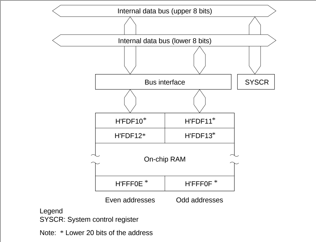
Figure 14-1 RAM Block Diagram (H8/3022 in Modes 1, 5, 6 and 7)
