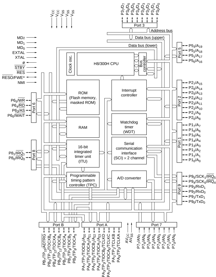
Figure 1-1 Block Diagram
