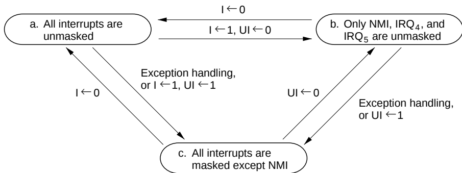
Figure 5-5 Interrupt Masking State Transitions (Example)
