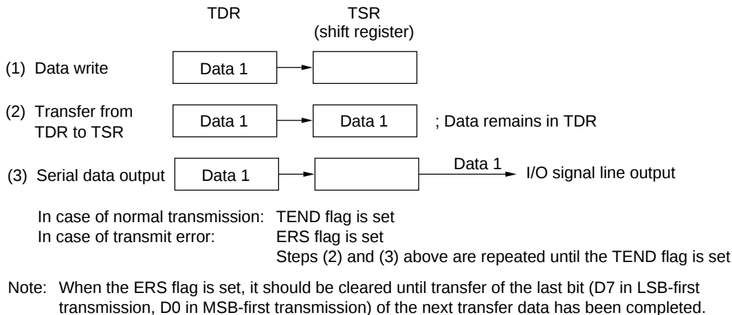
Figure 12-5 Relation Between Transmit Operation and Internal Registers
