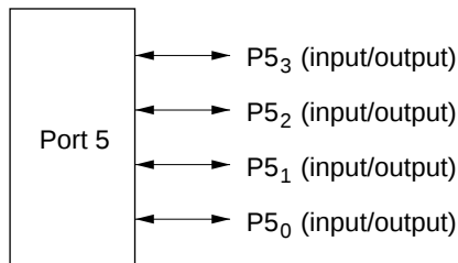
Figure 7-15 Pin Functions in Mode 7 (Port 5)
