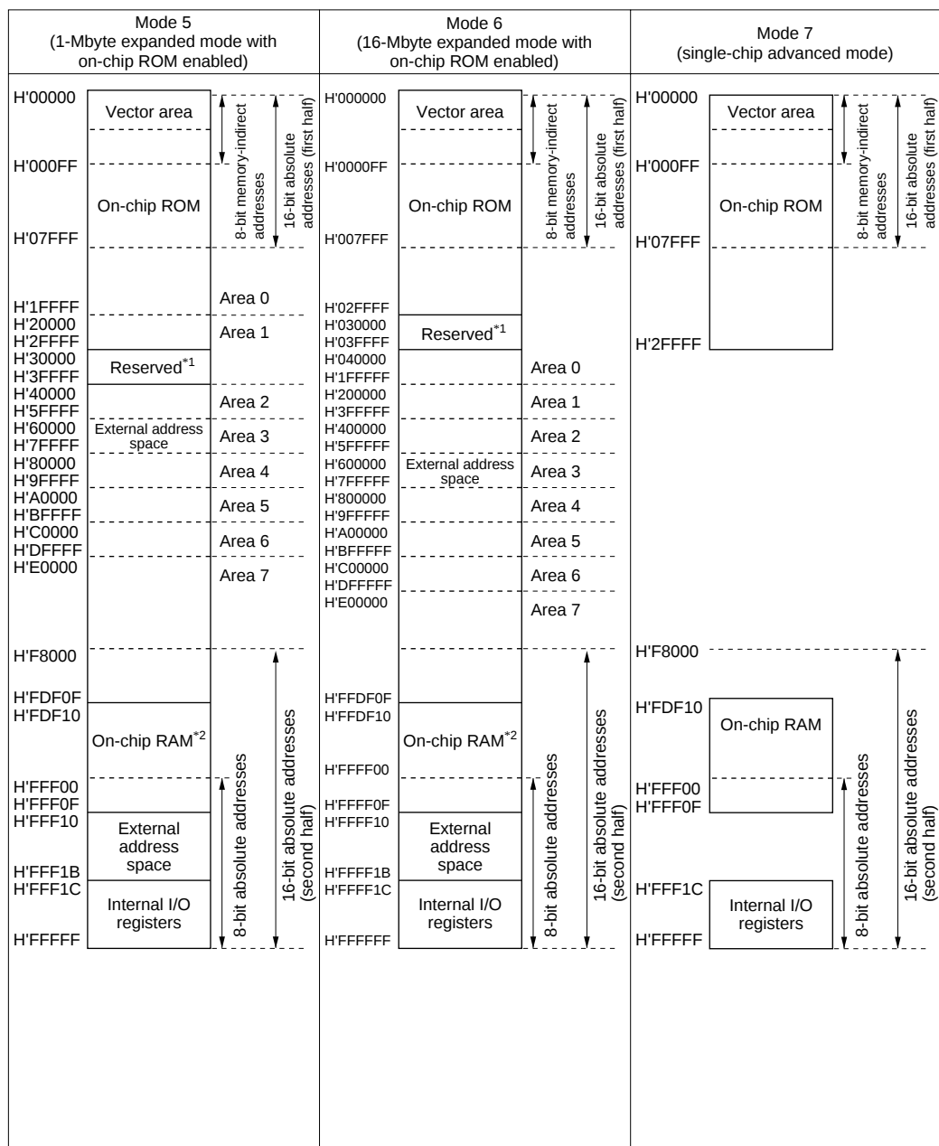
Figure 3-2 H8/3021 Memory Map in Each Operating Mode (2)
