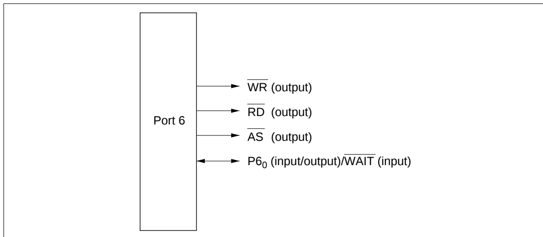
Figure 7-17 Pin Functions in Modes 1, 3, 5, and 6 (Port 6)
