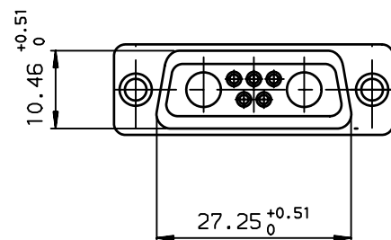
LAYOUT DIMENSIONS (after plating)
