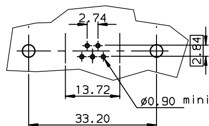
LAYOUT DIMENSIONS (after plating)
