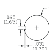
15/32 INCH BUSHING
