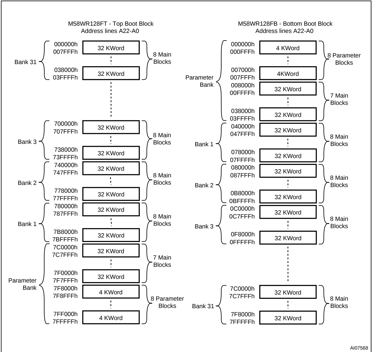
Figure 4. Memory Map
