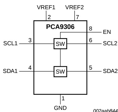
Fig 1. Logic diagram of PCA9306 (positive logic)
