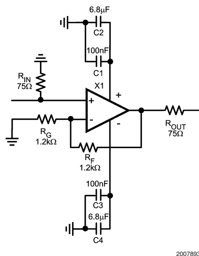
FIGURE 4. Typical Application with Suggested Supply Bypassing
