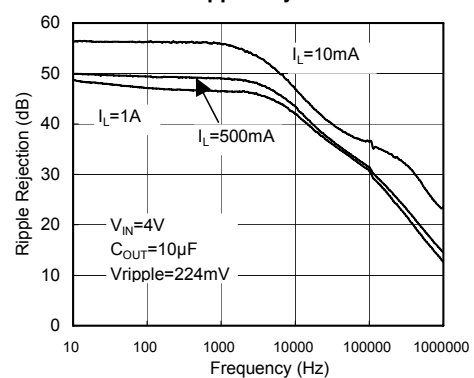
Ripple Rejection
