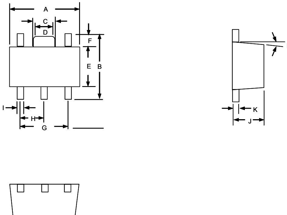
SOT-89-5 Package
