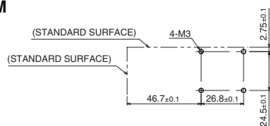
MOUNTING SCREW HOLES
