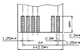
適用 FPC, FFC 寸法 RECOMMENDED APPLICABLE FPC LAYOUT
