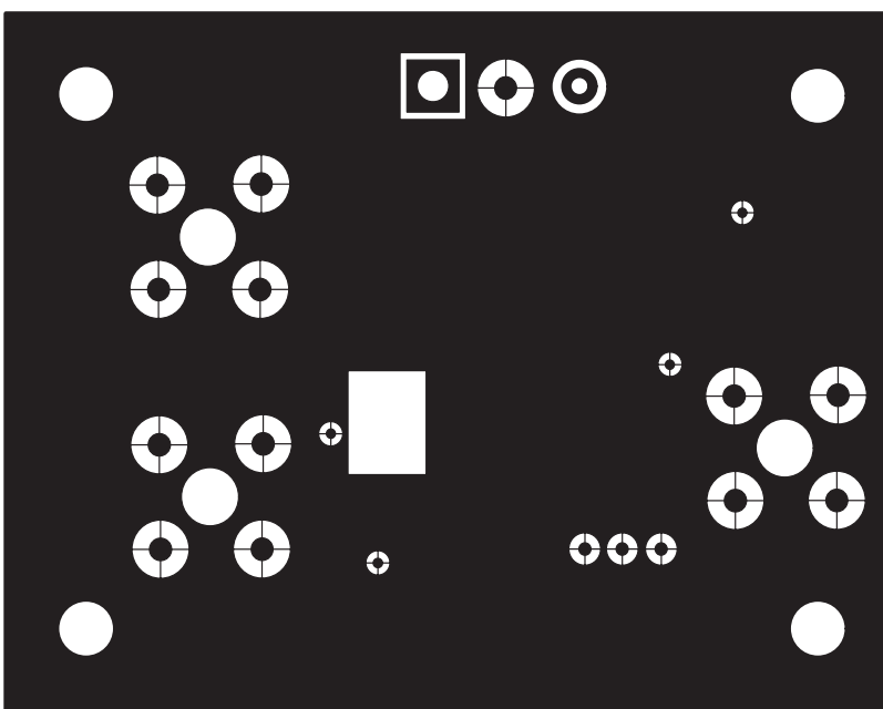
Figure 2–3. THS4021 EVM PC Board Layout – Back Side
