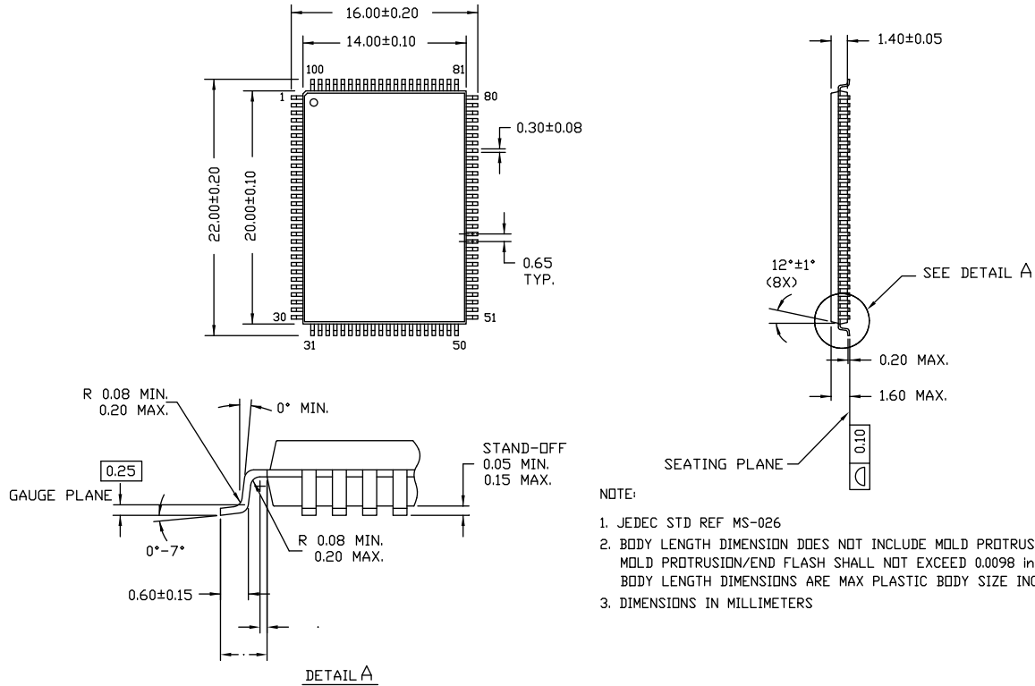
Figure 7. 100-pin TQFP (14 × 20 × 1.4 mm) A100RA Package Outline, 51-85050
