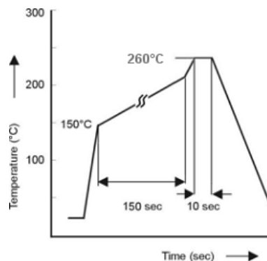
soldering condition
