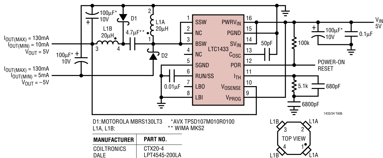
5V to \pm 5V Outputs
