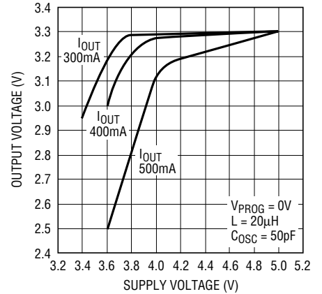
Dropout Characteristics at Different Load Currents ( V_{OUT} = 3.3\text{V} )
