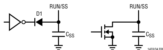
Figure 8. RUN/SS Pin Interfacing
