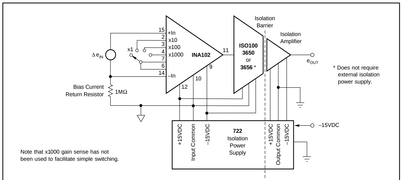
FIGURE 10. Precision Isolated Instrumentation Amplifier.
