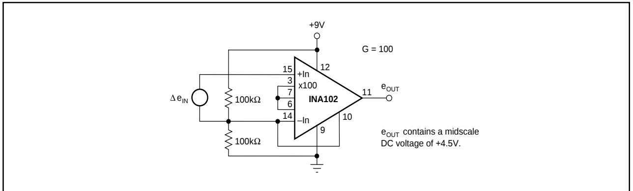
FIGURE 9. Single Supply Low Power Instrumentation Amplifier.
