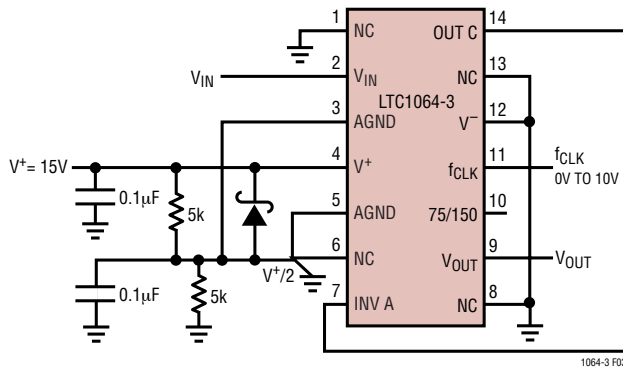
Figure 3. Single Supply Operation. If Fast Power Up or Down Transients are Expected, Use a 1N5817 Schottky Diode Between Pin 4 and Pin 5
