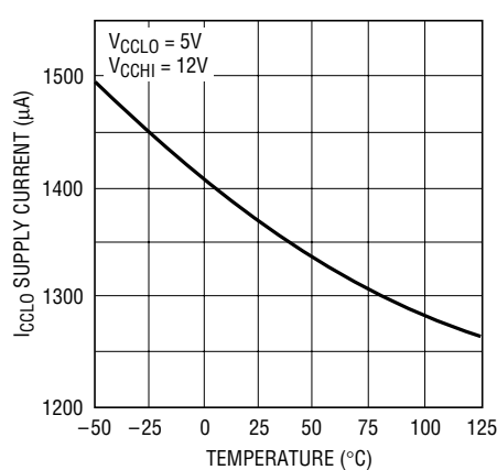
ICCLO Supply Current vs Temperature
