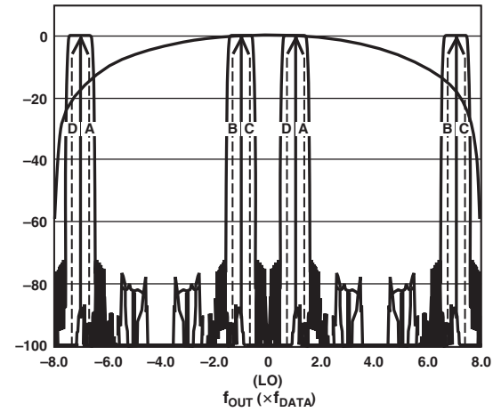
Figure 43. 8× Interpolation, Complex f_{DAC}/8 Modulation
