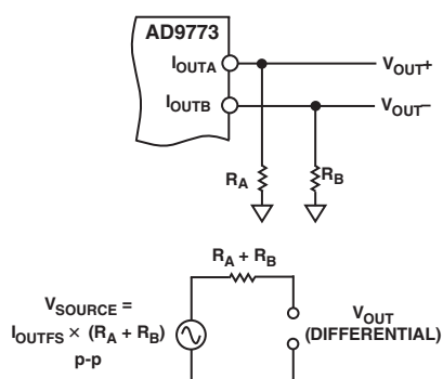
Figure 52. DAC Output Equivalent Circuit
