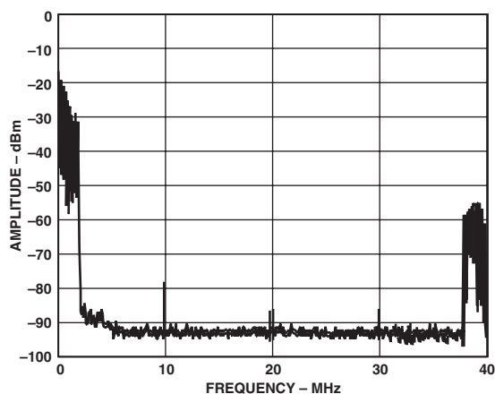
Figure 44. AD9773, Real DAC Output of Complex Input Signal Near Baseband (Positive Frequencies Only), Interpolation = 4x, No Modulation in AD9773
