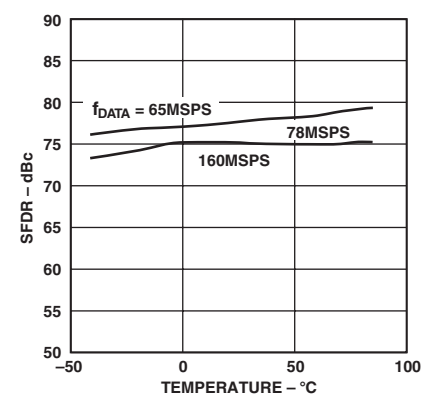
TPC 18. SFDR vs. Temperature @ f_{OUT} = f_{DATA}/11
