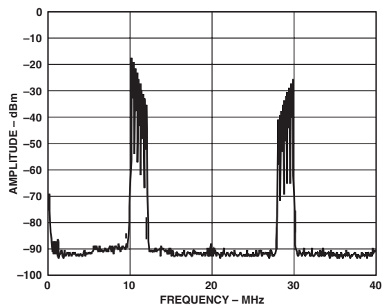
Figure 48. AD9773, Real DAC Output of Complex Input Signal Near Baseband (Negative Frequencies Only), Interpolation = 4\times , Complex Modulation in AD9773 = -f_{DAC}/4
