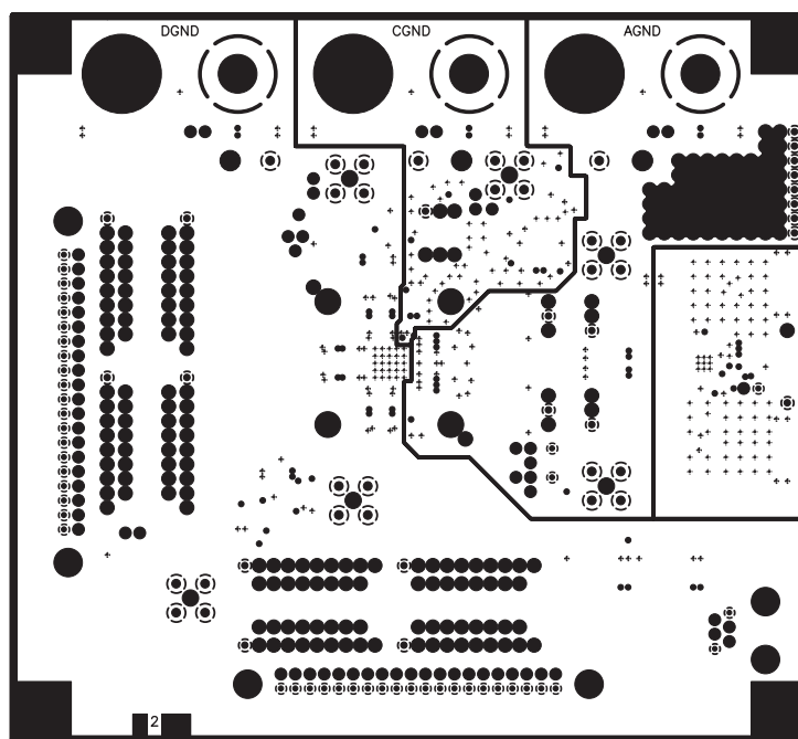
Figure 67. AD9773 Evaluation Board Layout, Layer Two (Ground Plane)
