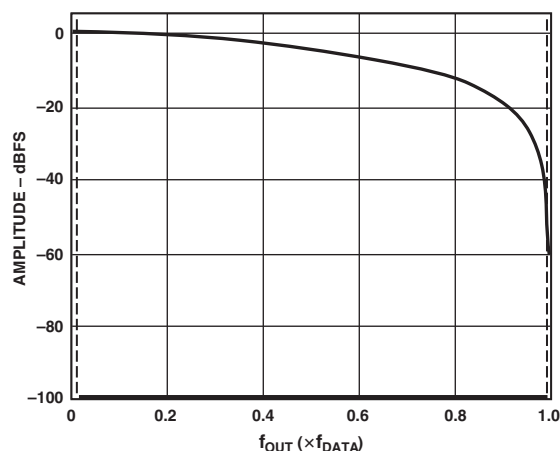
Figure 26a. No Interpolation, Modulation Disabled
