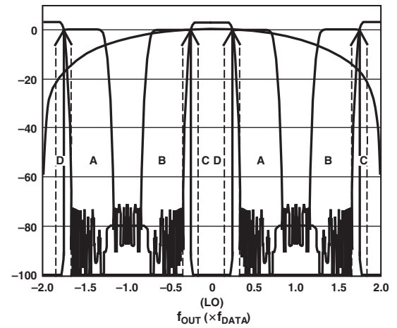
Figure 41. 2× Interpolation, Complex f_{DAC}/8 Modulation
