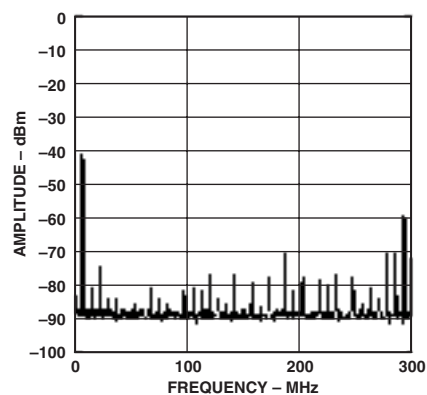
TPC 25. Single-Tone Spurious Performance, f_{OUT} = 10 MHz, f_{DATA} = 50 MSPS, Interpolation = 8x
