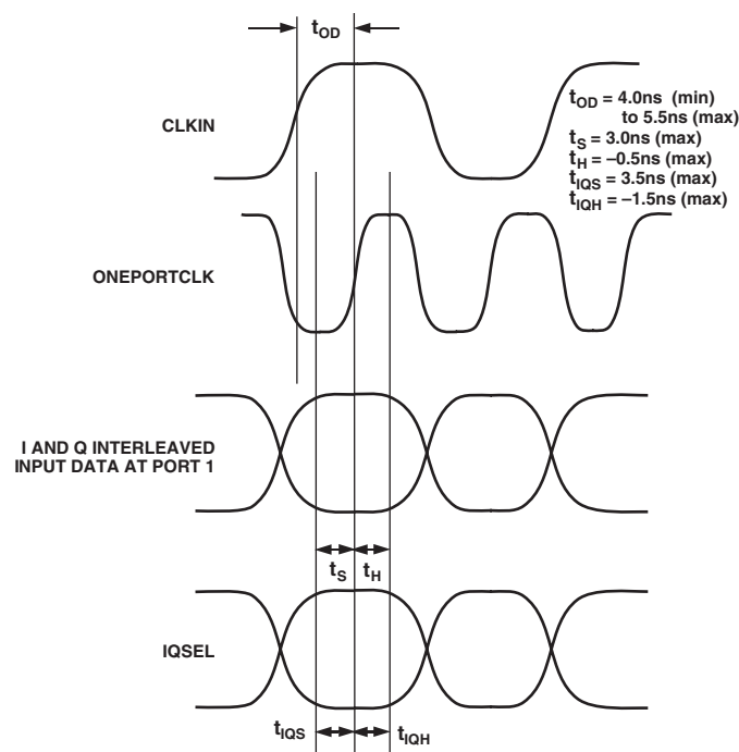
Figure 21. Timing Requirements in One Port Input Mode, with the PLL Enabled
