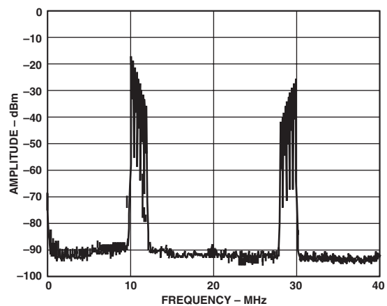
Figure 46. AD9773, Real DAC Output of Complex Input Signal Near Baseband (Positive Frequencies Only), Interpolation = 4x, Complex Modulation in AD9773 = +f_{DAC}/4
