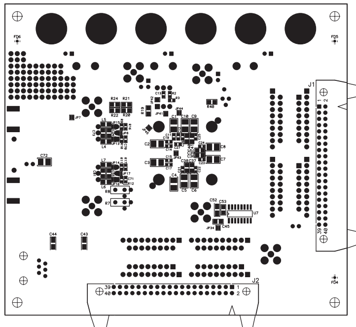
Figure 65. AD9773 Evaluation Board Components, Bottom Side
