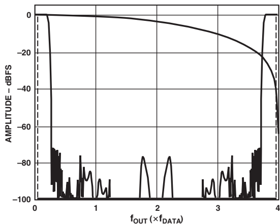
Figure 29a. 8× Interpolation, Modulation Disabled
