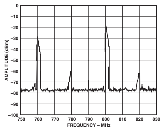
Figure 47. AD9773 Complex Output from Figure 46, Now Quadrature Modulated by AD8345 (LO = 800 MHz)
