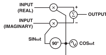
Figure 33. Quadrature Modulator
