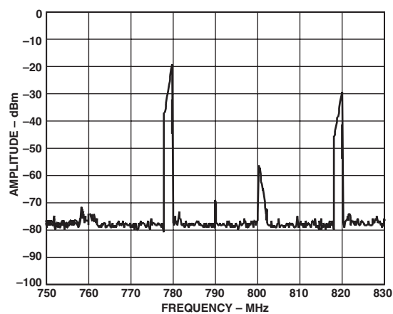
Figure 49. AD9773 Complex Output from Figure 48, Now Quadrature Modulated by AD8345 (LO = 800 MHz)
