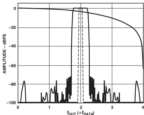
Figure 29b. 8× Interpolation, Modulation = f_{DAC}/2
