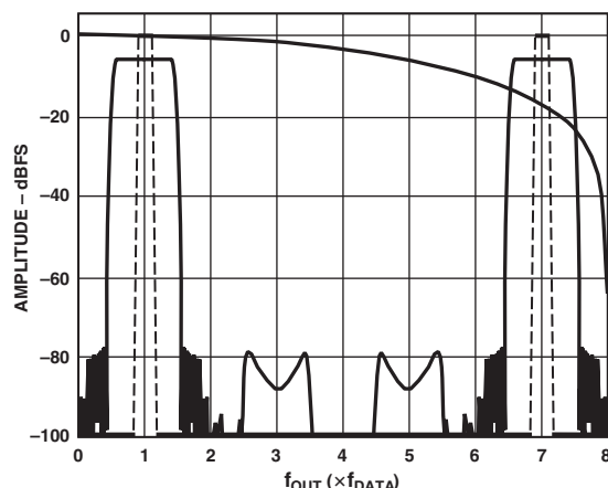
Figure 29d. 8× Interpolation, Modulation = f_{DAC}/8
