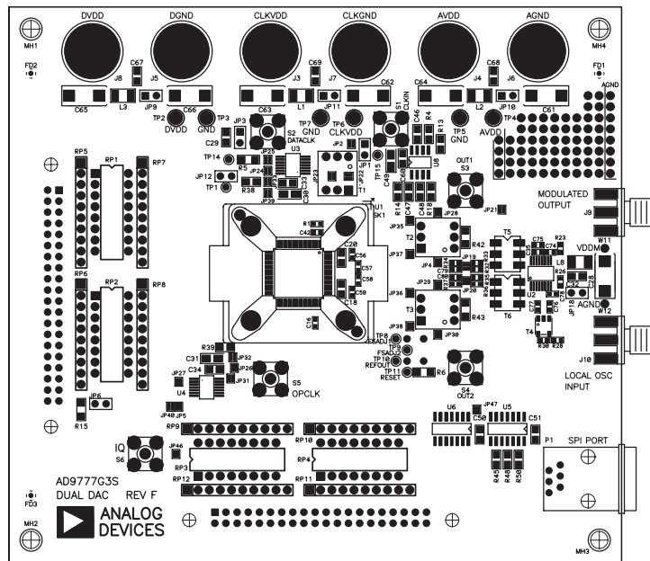
Figure 64. AD9773 Evaluation Board Components, Top Side
