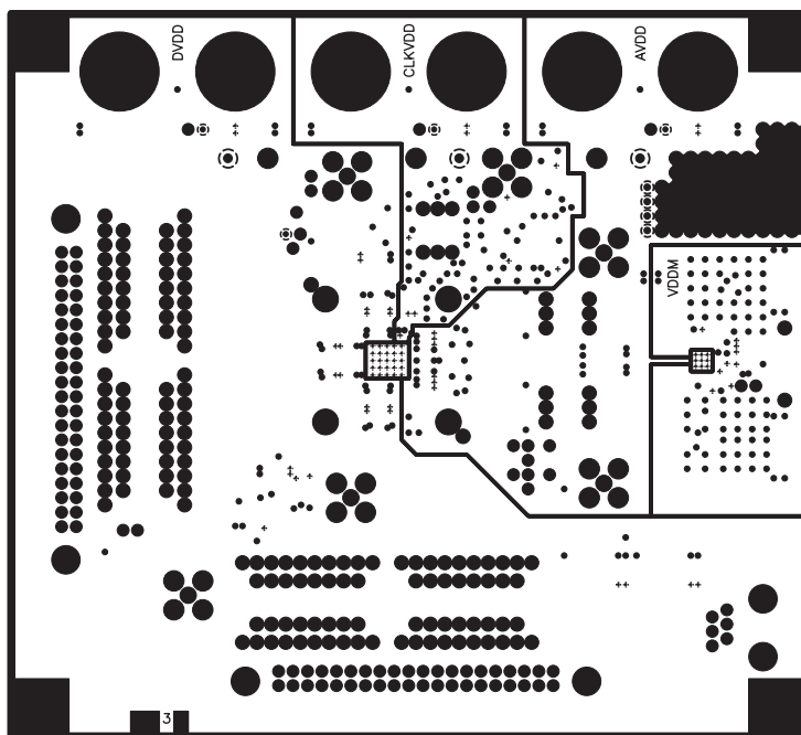
Figure 68. AD9773 Evaluation Board Layout, Layer Three (Power Plane)
