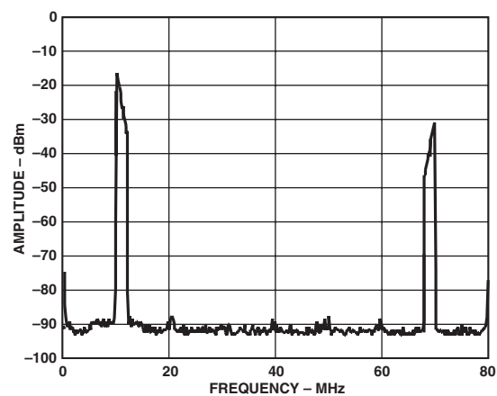
Figure 50. AD9773, Real DAC Output of Complex Input Signal Near Baseband (Positive Frequencies Only), Interpolation = 8\times , Complex Modulation in AD9773 = +f_{DAC}/8
