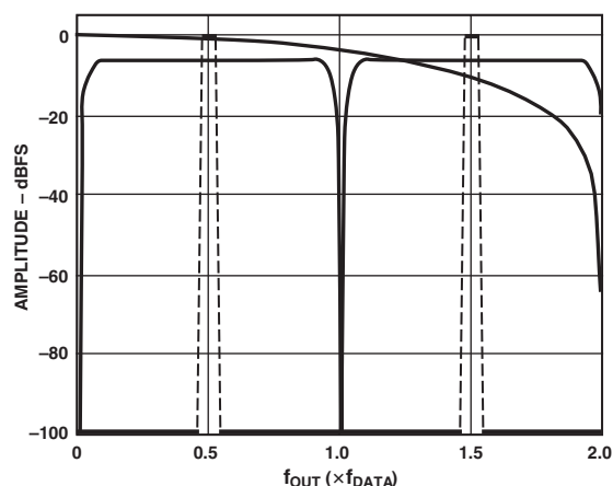
Figure 27c. 2× Interpolation, Modulation = f_{DAC}/4
