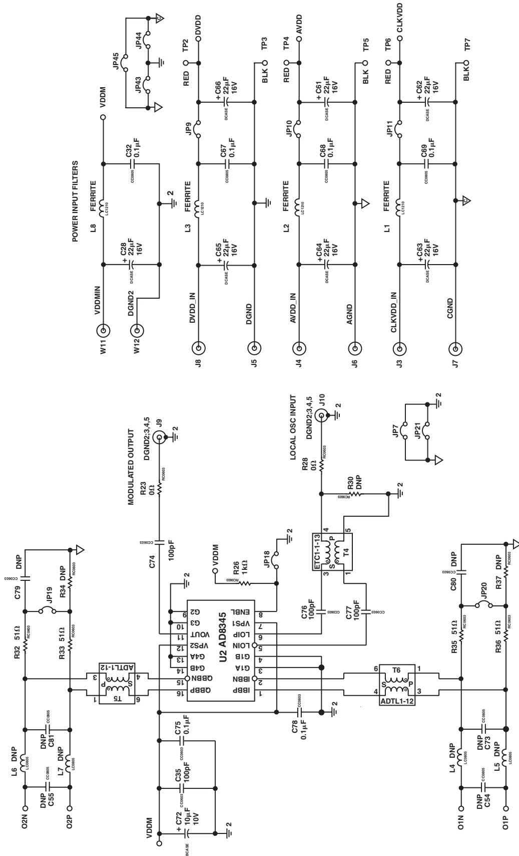
Figure 60. AD8345 Circuitry on AD9773 Evaluation Board
