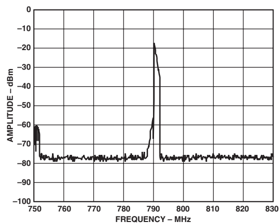
Figure 45. AD9773 Complex Output from Figure 44, Now Quadrature Modulated by AD8345 (LO = 800 MHz)
