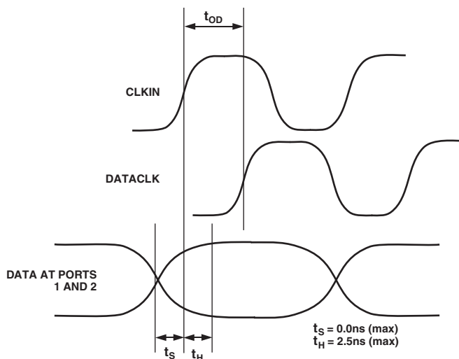
Figure 19. Timing Requirements in Two Port Input Mode, with PLL Enabled
