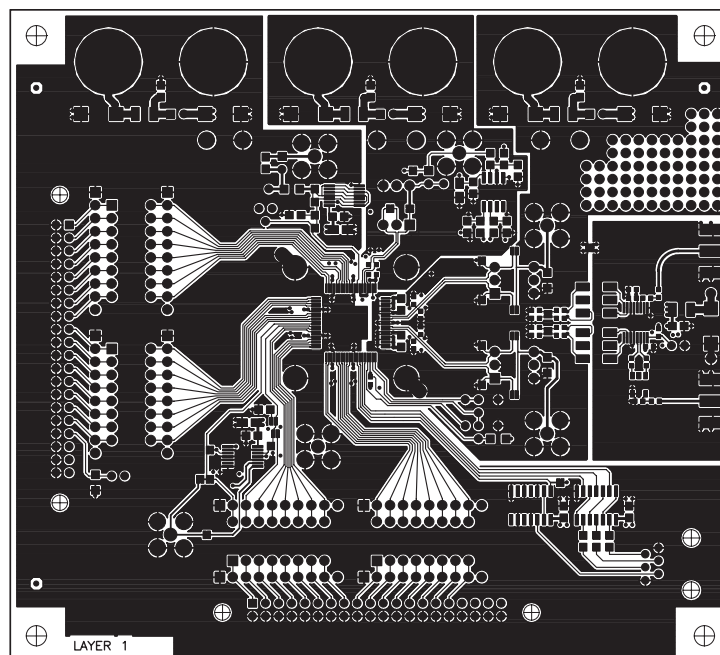
Figure 66. AD9773 Evaluation Board Layout, Layer One (Top)
