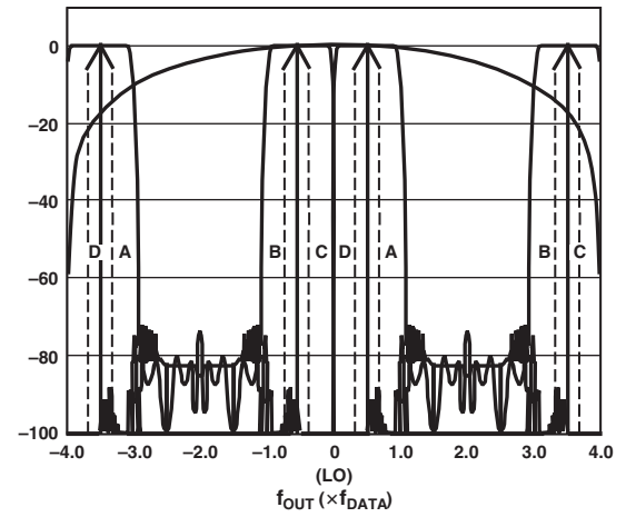
Figure 42. 4× Interpolation, Complex f_{DAC}/8 Modulation
