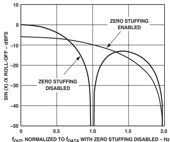
Figure 30. Effect of Zero Stuffing on DAC's \text{SIN}(x)/x Response
