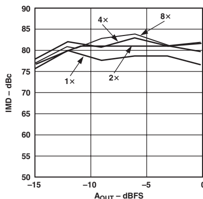
TPC 14. Third Order IMD Products vs. A_{OUT} and Interpolation Rate f_{DATA} = 50 MSPS for All Cases, 1 \times f_{DAC} = 50 MSPS 2 \times f_{DAC} = 100 MSPS 4 \times f_{DAC} = 200 MSPS 8 \times f_{DAC} = 400 MSPS
