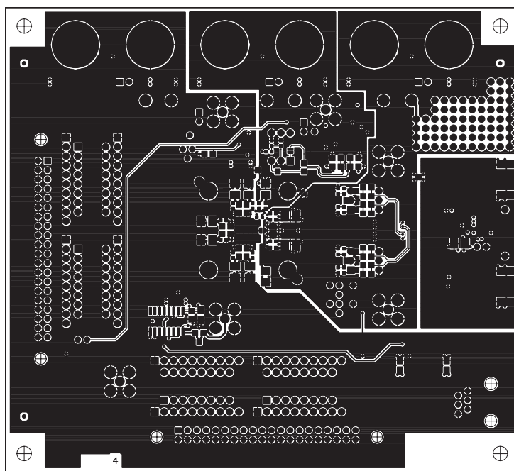
Figure 69. AD9773 Evaluation Board Layout, Layer Four (Bottom)
