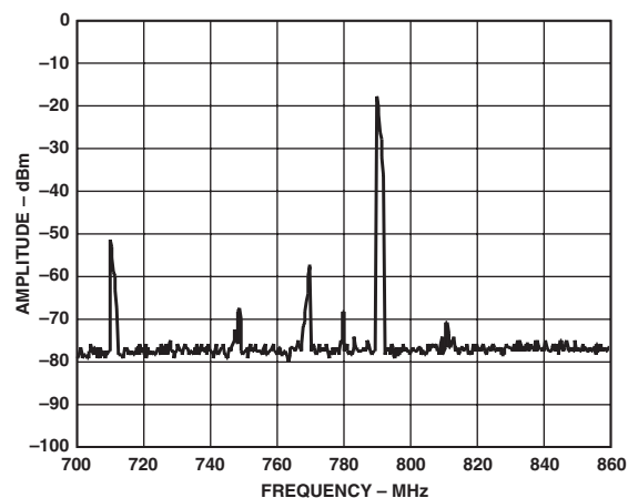
Figure 51. AD9773 Complex Output from Figure 50, Now Quadrature Modulated by AD8345 (LO = 800 MHz)
