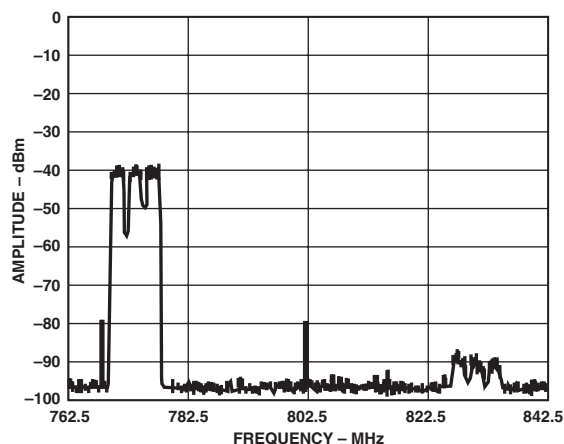
Figure 55. AD9773/AD8345 Synthesizing a Three-Carrier WCDMA Signal at an LO of 800 MHz
