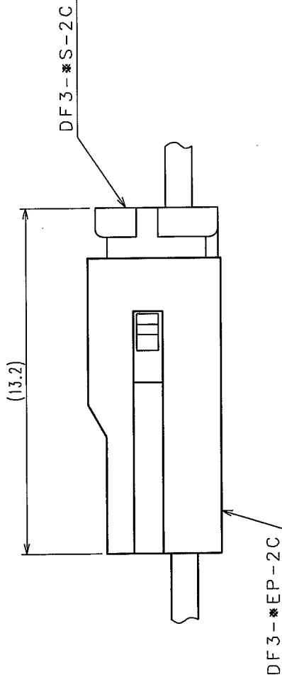
MATED CONNECTORS
