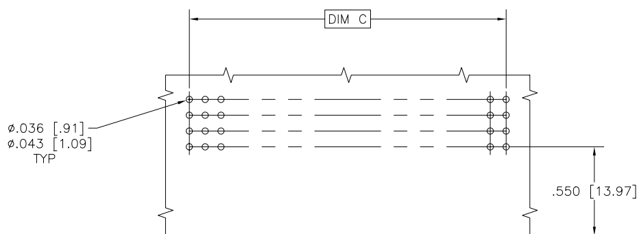
SECTION X-X
