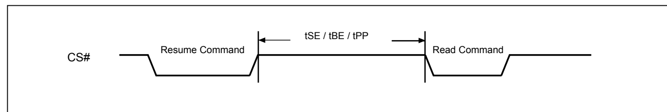
Figure 70. Resume to Read Latency
