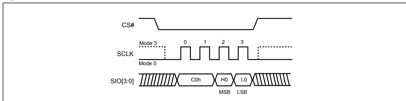
Figure 34. QPI Mode
