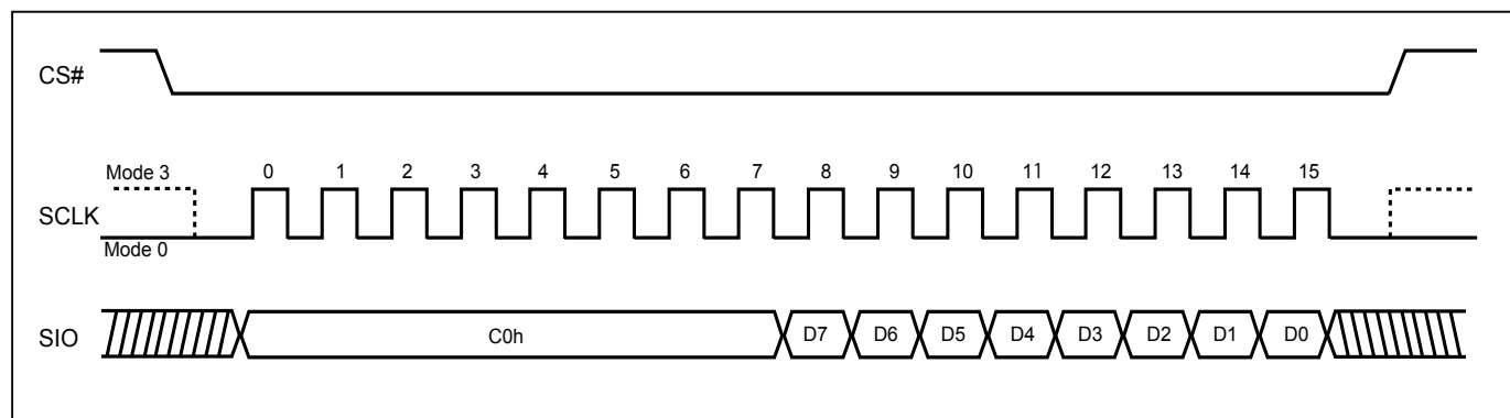
Figure 33. SPI Mode
