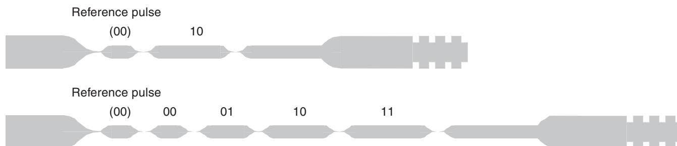
Figure 5-15. 1-of-4-coding Protocol
