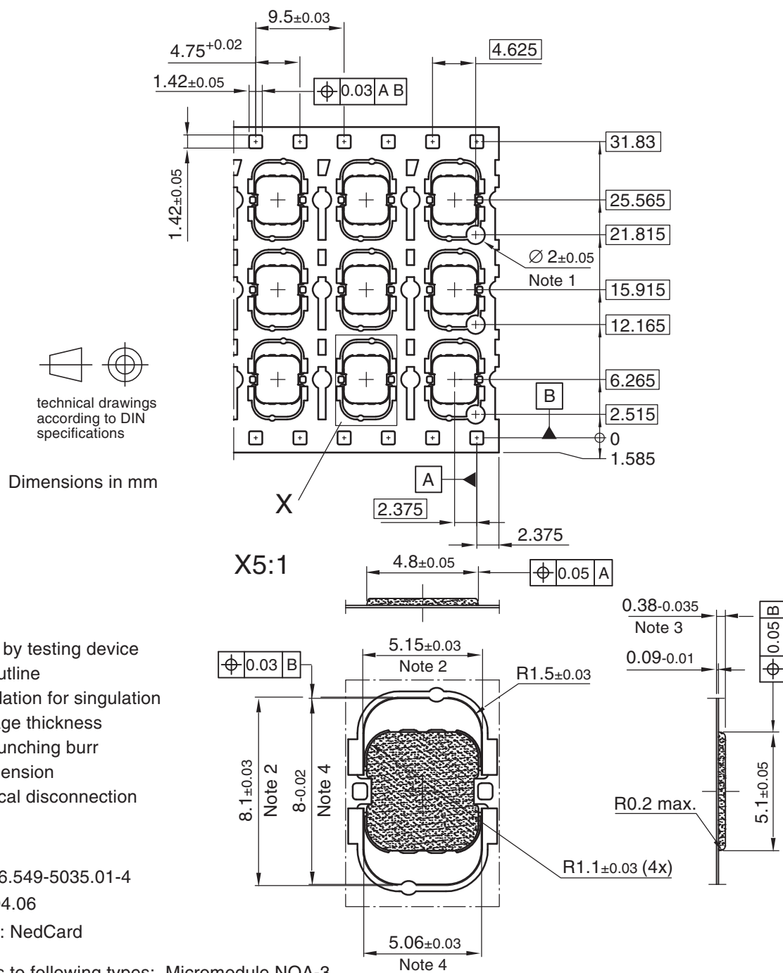
Figure 11-6. NOA3 Micromodule
