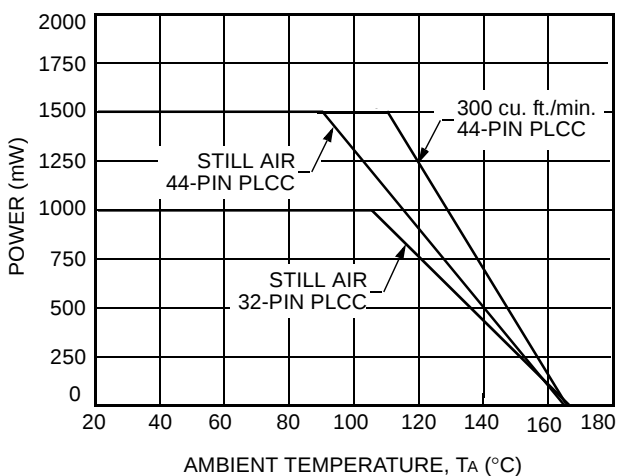
Figure 21. Power Derating
