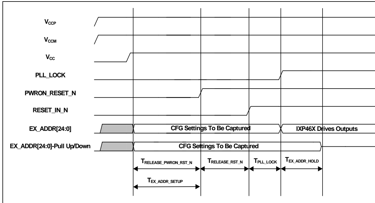
Figure 49. Reset Timings
