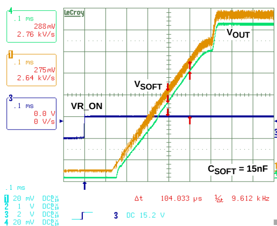
FIGURE 7. SOFT-START WAVEFORM SHOWING SLEW RATE OF 2.5mV/μs AT V_{SEL} = 1.4375V , I_{LOAD} = 10A
