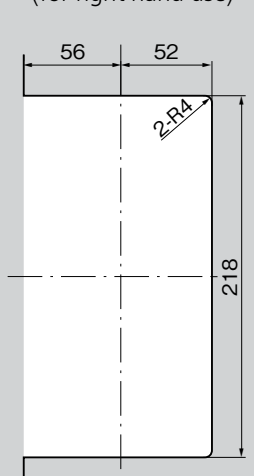
パネル穴明け寸法 (右開き用) Panel drilling dimensions (for right-hand use)
