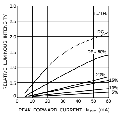
Fig. 30 Luminous intensity vs. peak forward current
