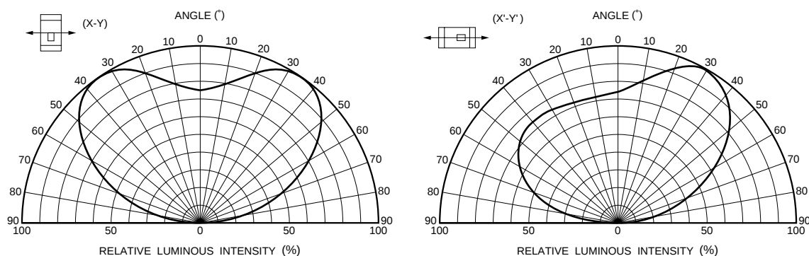
Fig. 1 Directional pattern
