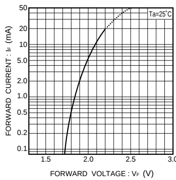
Fig. 26 Forward current vs. forward voltage
