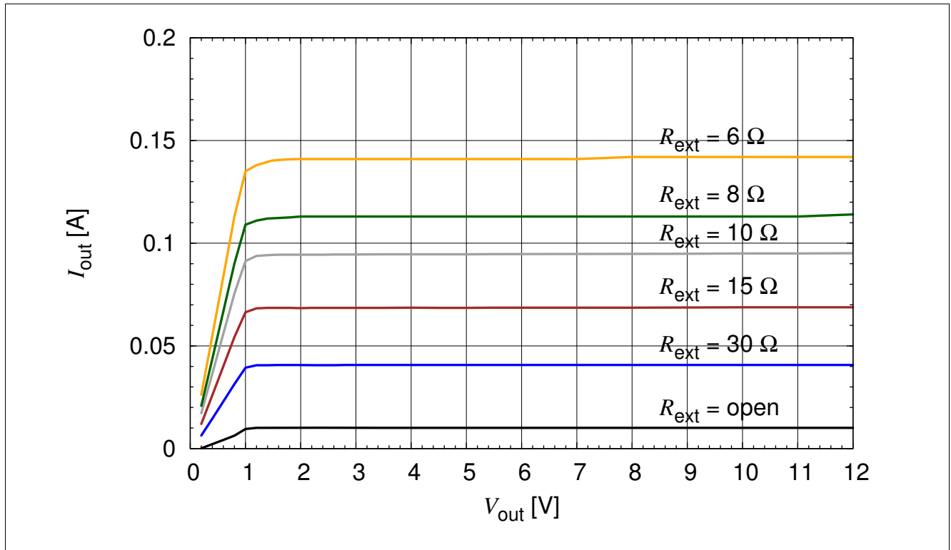
Figure 3-4 BCR420U: Output Current versus V_{out} I_{out} = f(V_{out}) , V_{EN} = 40\text{ V} , R_{ext} = \text{Parameter}
