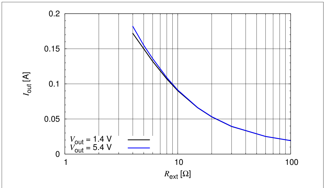
Figure 3-5 BCR420U: Output Current versus R_{ext} I_{out} = f(R_{ext}) , V_{EN} = 40\text{ V} , V_{out} = \text{Parameter}
