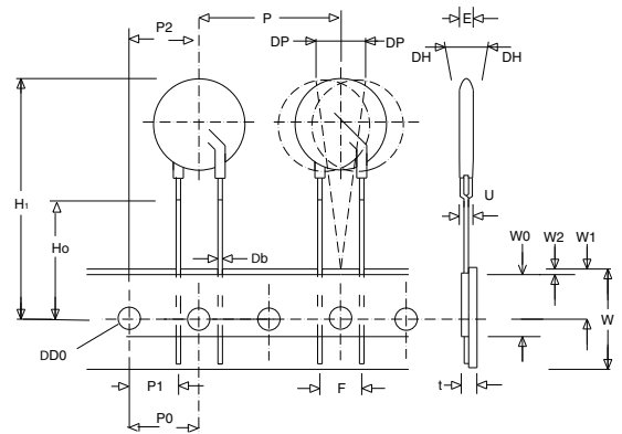
UNDER CRIMPED LEADS "ZU"
