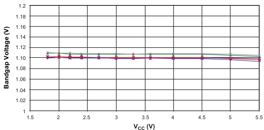
Figure 29-19. ATmega164P-B: Calibrated Bandgap Voltage versus V_{CC}
