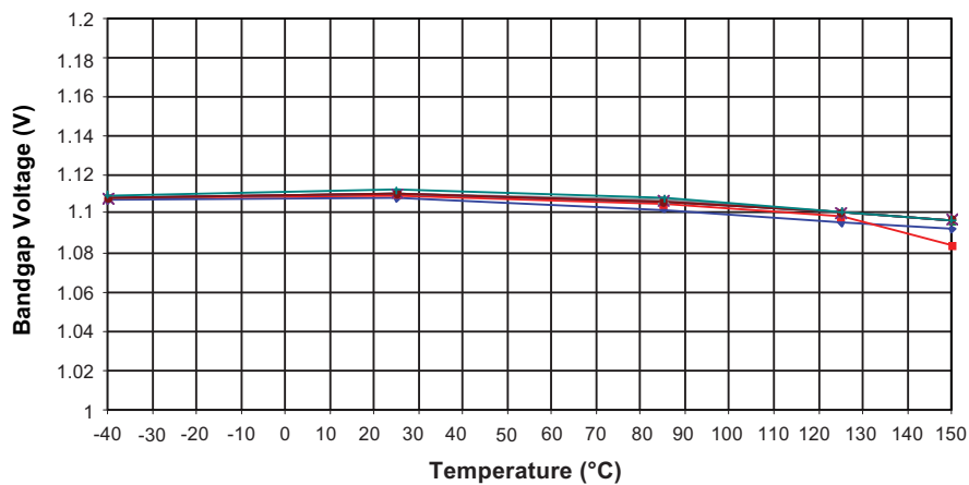
Figure 29-20. ATmega164P-B: Bandgap Voltage versus Temperature
