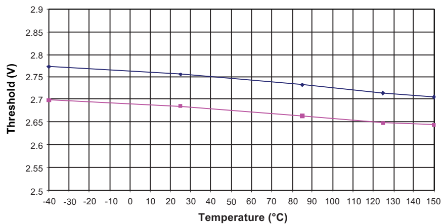
Figure 29-18. ATmega164P-B: BOD Threshold versus Temperature ( V_{BOT} = 2.7V )
