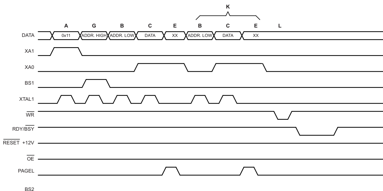
Figure 27-4. Programming the EEPROM Waveforms
