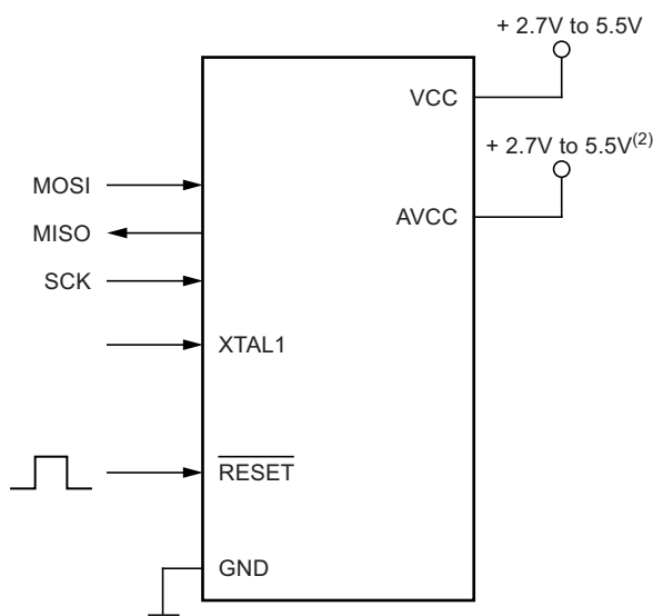
Figure 27-10. Serial Programming and Verify (1)
