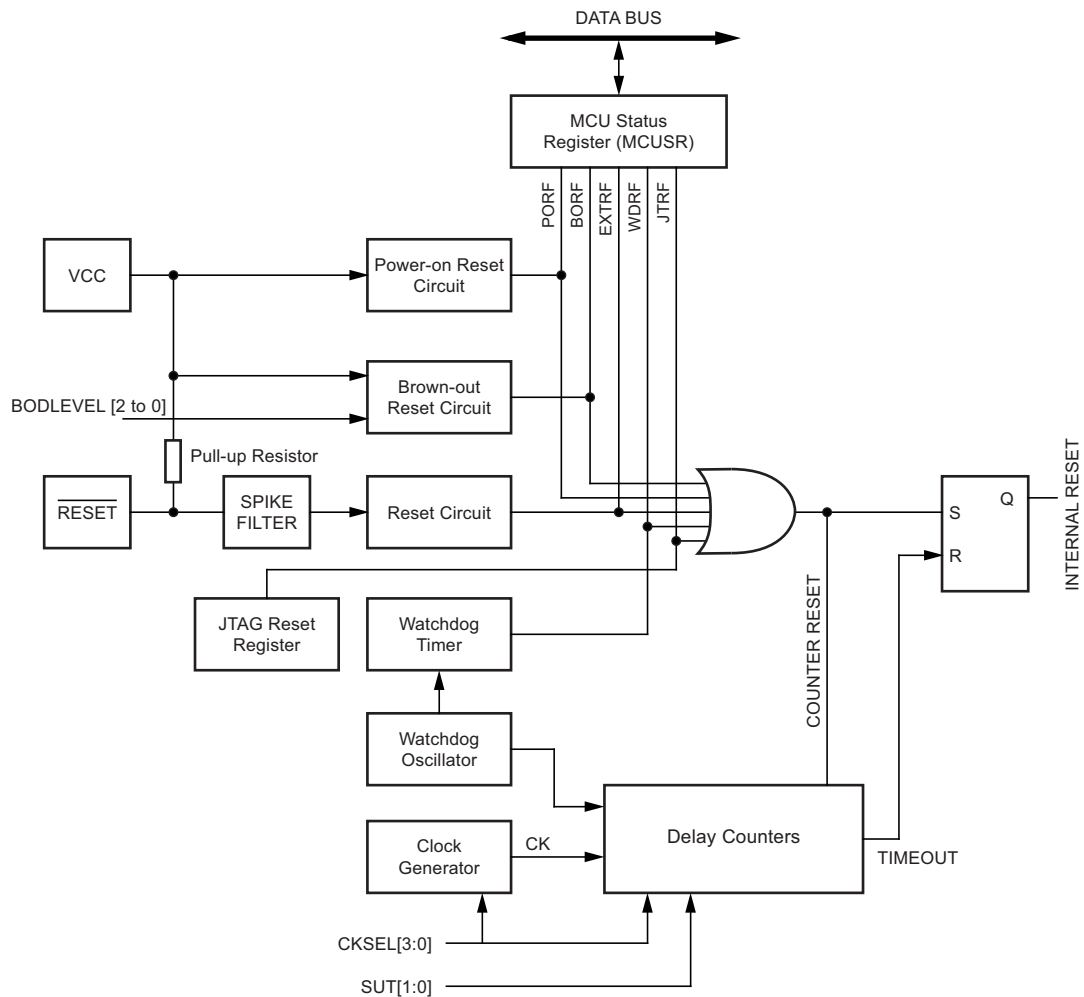
Figure 11-1. Reset Logic
