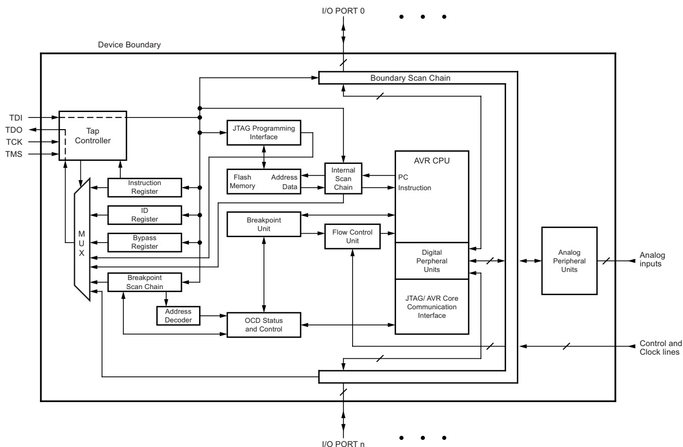
Figure 24-1. Block Diagram
