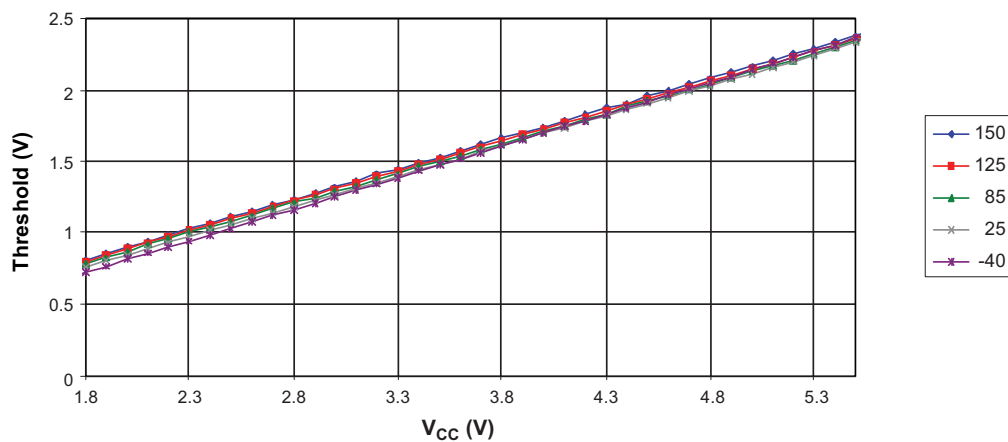
Figure 29-66. ATmega644P-B: Reset Pin Input Threshold versus V_{CC} ( V_{IL} , I/O Pin Read as '0')
