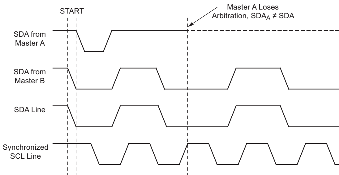
Figure 21-8. Arbitration Between Two Masters
