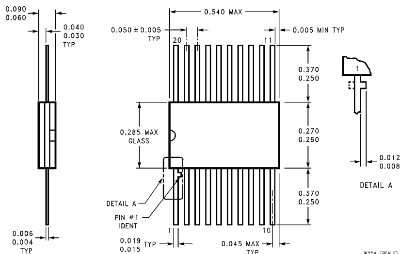
20-Lead Ceramic Flat Package (W) Order Number 54LS244FMQB Package Number W20A
