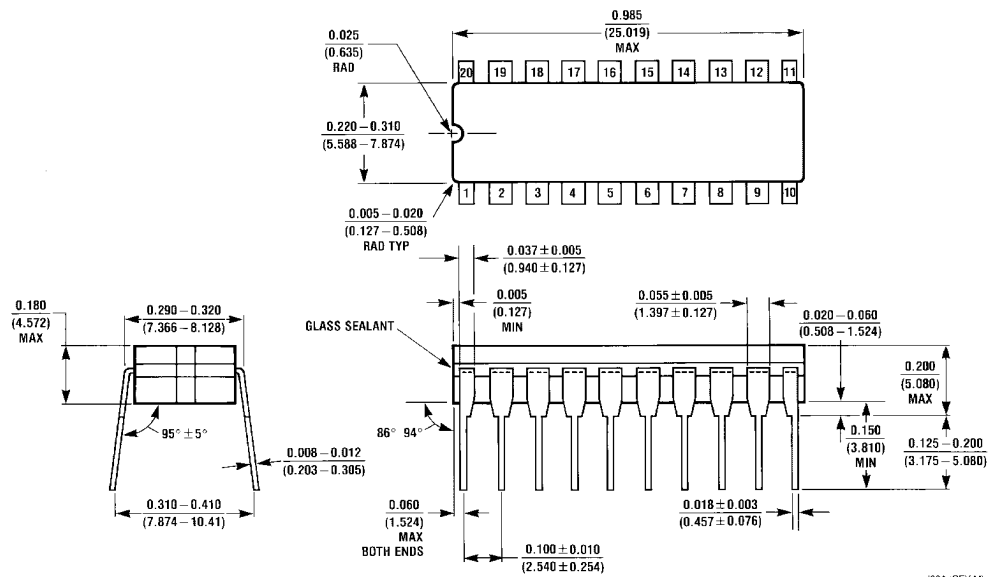
20-Lead Ceramic Dual-In-Line Package (J) Order Number 54LS244DMQB Package Number J20A
