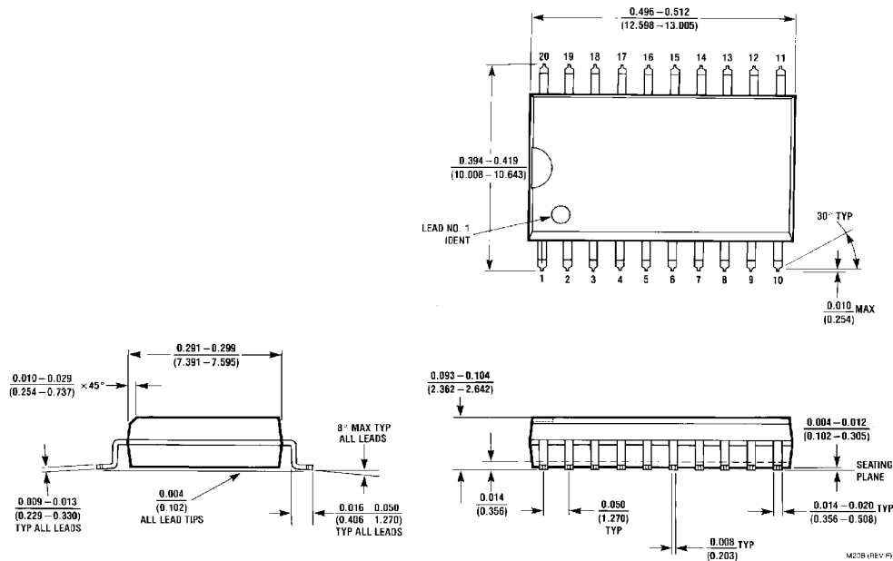
20-Lead Wide Small Outline Molded Package (M) Order Number DM74LS244WM Package Number M20B
