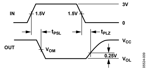
Figure 29. Driver Enable and Disable Times ( t_{PZL} , t_{PSL} , t_{PLZ} )
