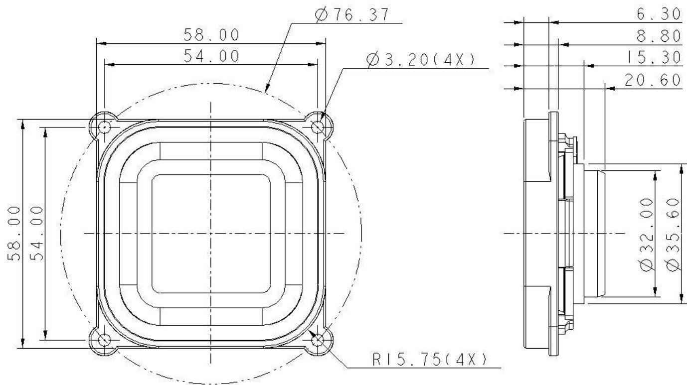
Figure 2. Nominal dimensions
