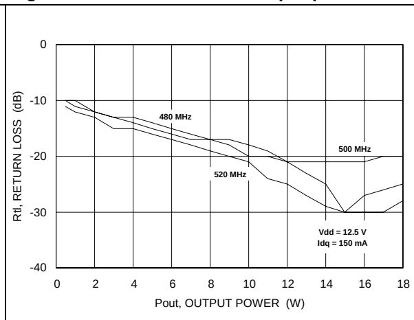
Figure 19. Return loss vs. output power
