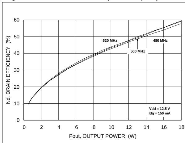
Figure 18. Drain efficiency vs. output power
