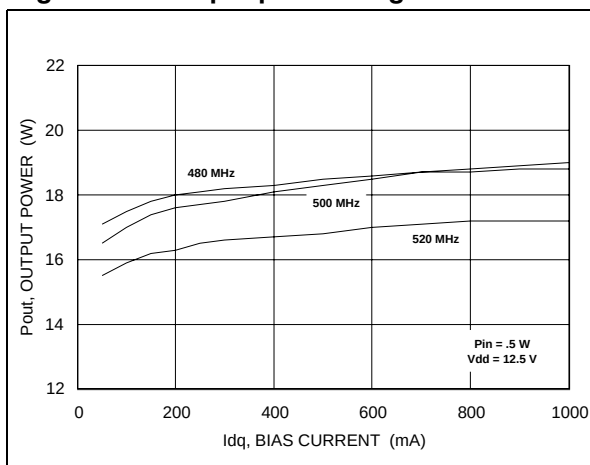
Figure 20. Output power vs. gate bias current
