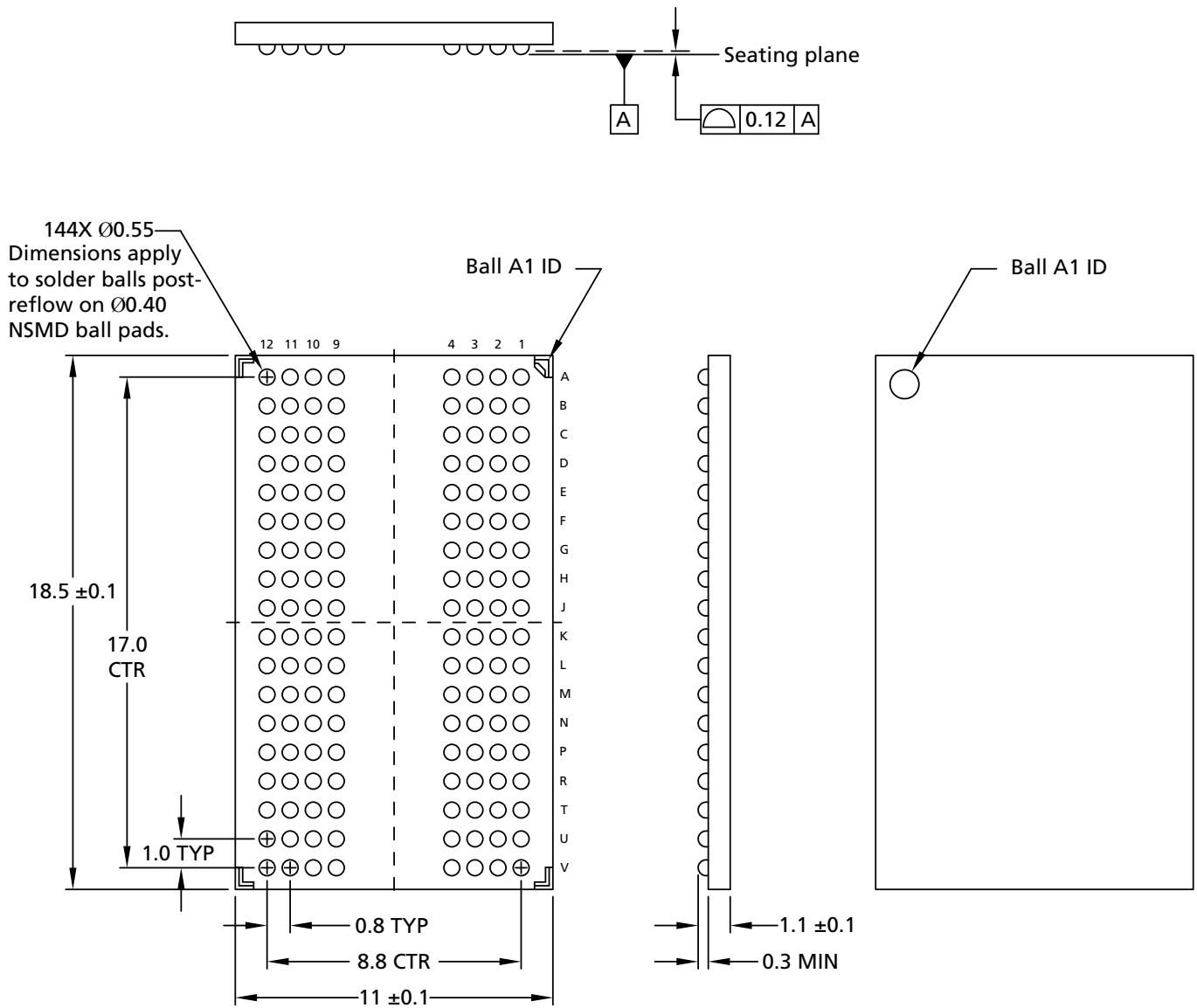
Figure 5: 144-Ball FBGA
