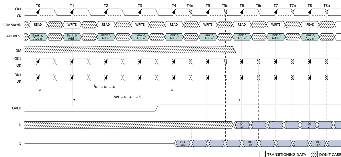
Figure 26: READ/WRITE Interleave
