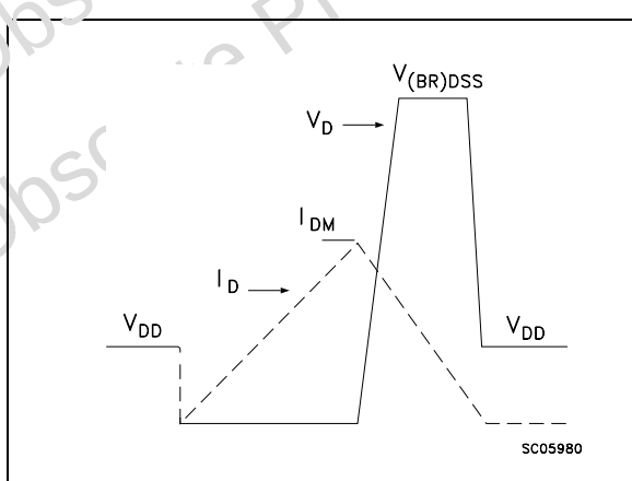
Figure 19. Unclamped inductive waveform
