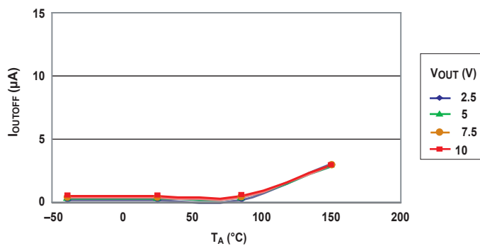
Output Leakage Current (Off) versus Ambient Temperature
