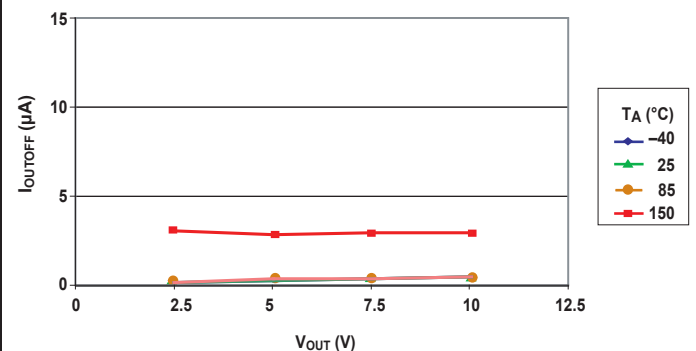
Output Leakage Current (Off) versus Output Voltage
