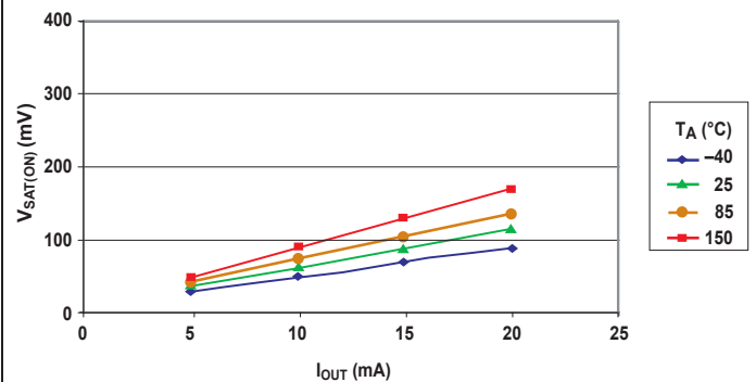
Output Voltage (On) versus Output Current
