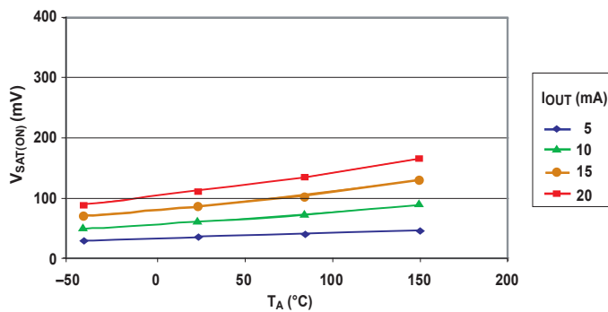
Output Voltage (On) versus Ambient Temperature
