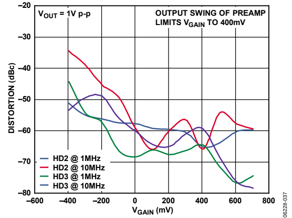
Figure 37. 2 nd and 3 rd Harmonic Distortion vs. V_{GAIN} at 1 MHz and 10 MHz
