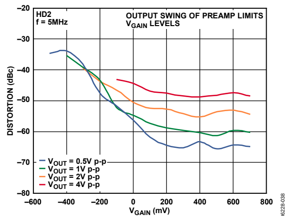
Figure 38. 2 nd Harmonic Distortion vs. V_{GAIN} for Four Values of Output Voltage ( V_{OUT} )
