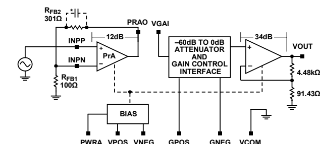
Figure 77. Simplified Block Diagram
