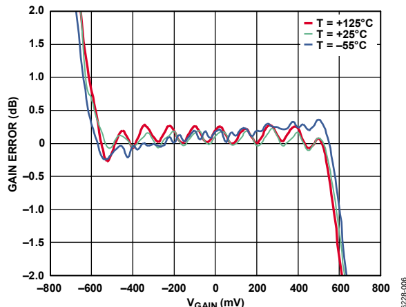
Figure 6. Gain Error vs. V_{\text{GAIN}} for Three Values of Temperature (T)
