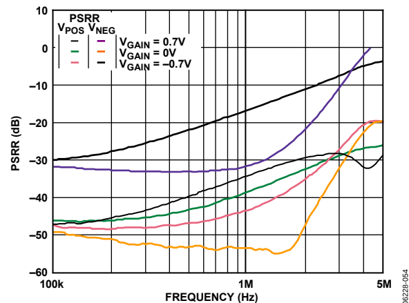
Figure 54 PSRR vs. Frequency for Three Values of V_{\text{GAIN}}
