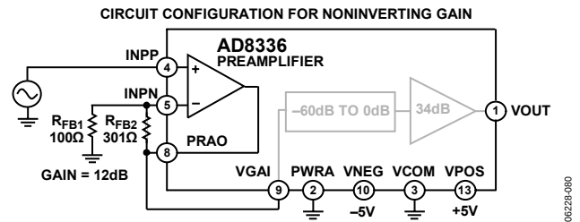
Figure 80. Circuit Configuration for Noninverting Gain
