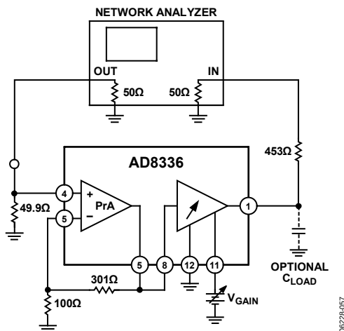
Figure 57. Frequency Response
