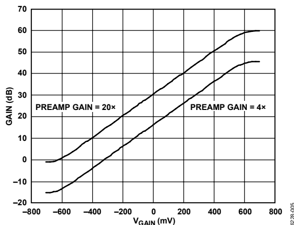
Figure 5. Gain vs. V_{\text{GAIN}} for Preamp Gains of 4\times and 20\times
