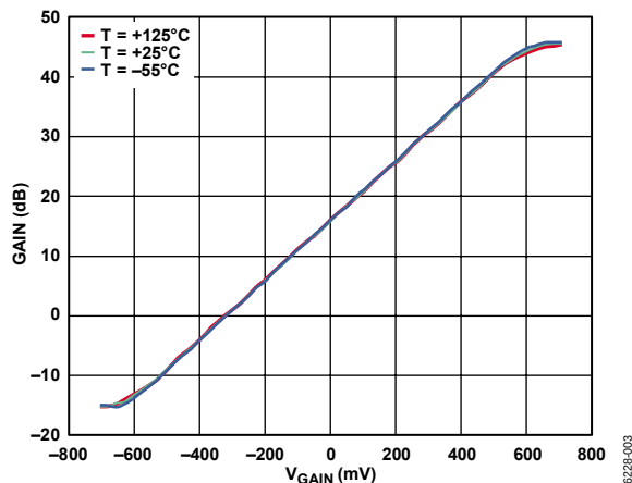
Figure 3. Gain vs. V_{\text{GAIN}} for Three Values of Temperature (T)
