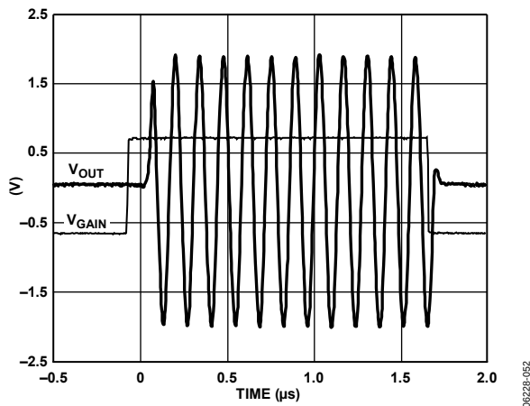
Figure 52. Gain Response
