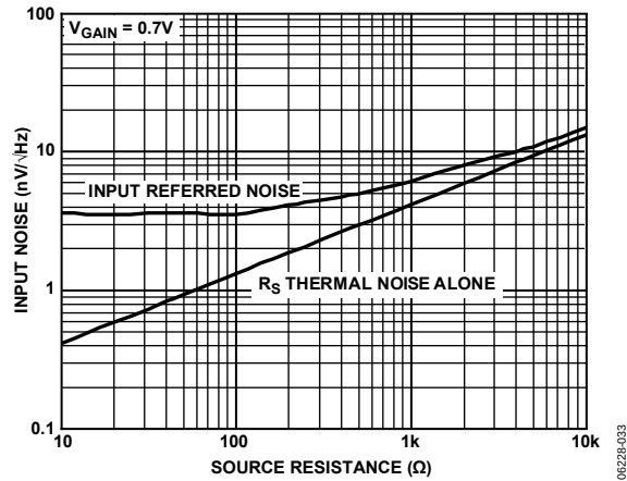
Figure 33. Input Referred Noise vs. Source Resistance
