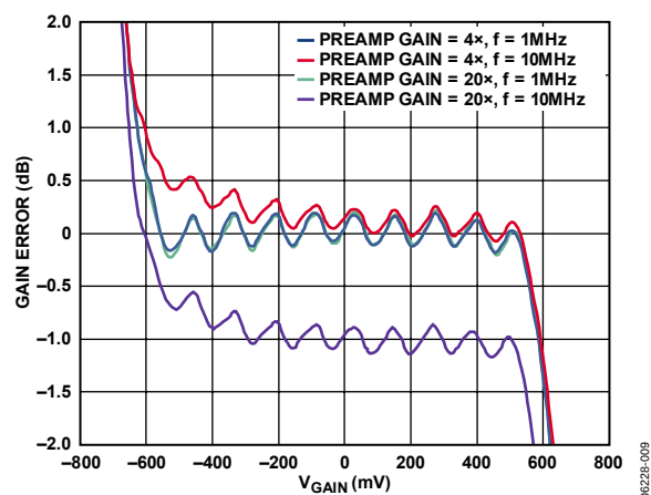
Figure 9. Gain Error vs. V_{\text{GAIN}} at 1 MHz and 10 MHz and for Preamp Gains of 4x and 20x
