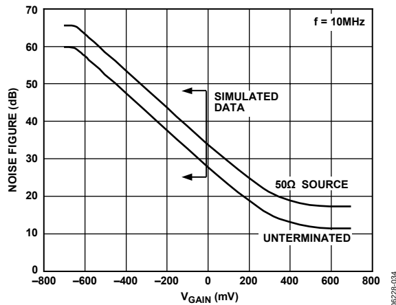
Figure 34. Noise Figure vs. V_{GAIN}
