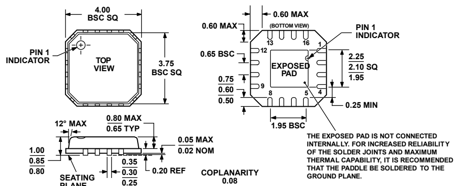
Figure 90. 16-Lead Lead Frame Chip Scale Package [LFCSP_VQ] 4 mm × 4 mm Body, Very Thin Quad (CP-16-4)
