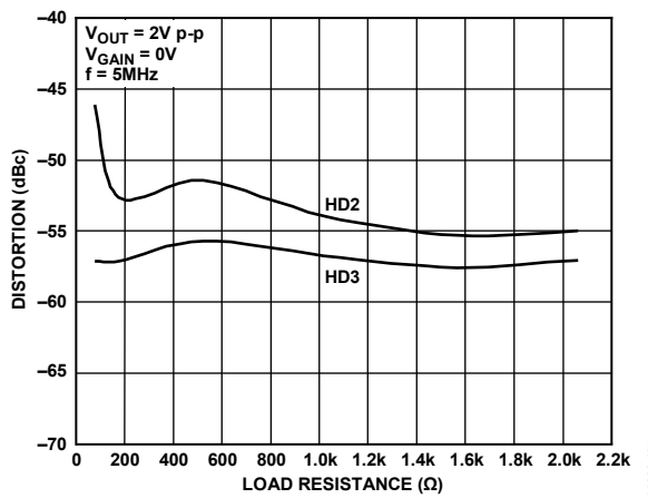
Figure 35. Harmonic Distortion vs. Load Resistance
