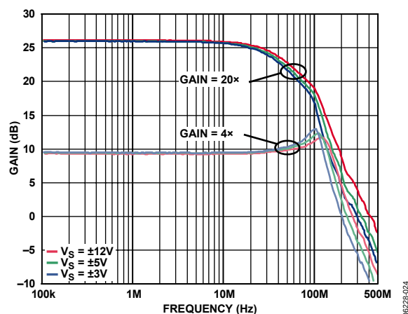
Figure 24. Preamp Frequency Response for Three Values of Supply Voltage ( V_S ) and Inverting Gain Values of -3\times and -19\times
