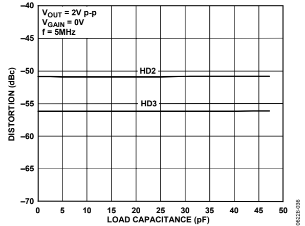
Figure 36. Harmonic Distortion vs. Load Capacitance
