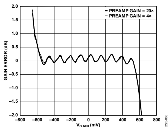
Figure 8. Gain Error vs. V_{\text{GAIN}} for Preamp Gains of 4\times and 20\times
