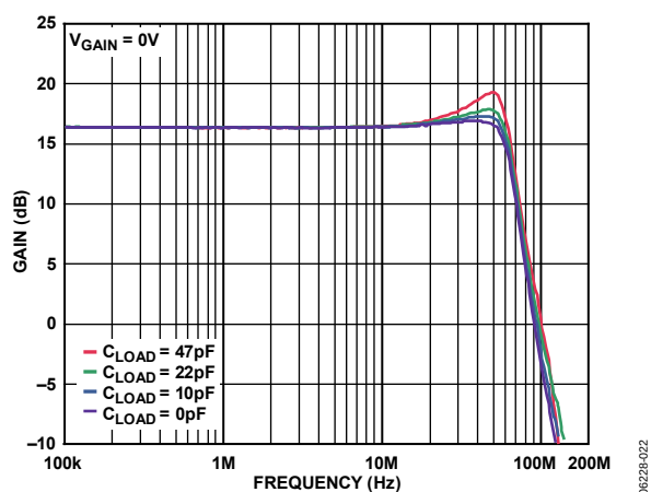
Figure 22. Frequency Response for Various Values of Load Capacitance ( C_{\text{LOAD}} )
