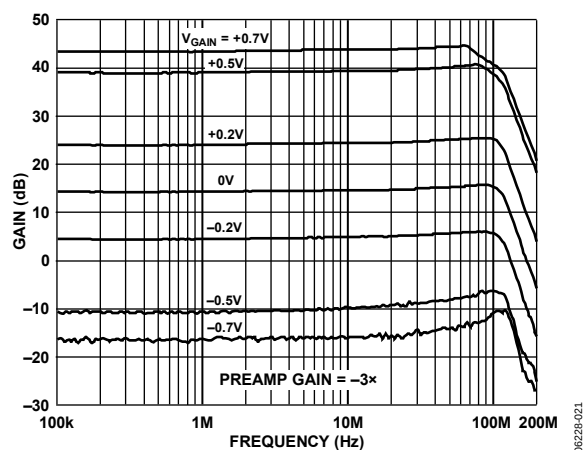
Figure 21. Frequency Response for Various Values of V_{\text{GAIN}} for Preamp Gain of -3\times
