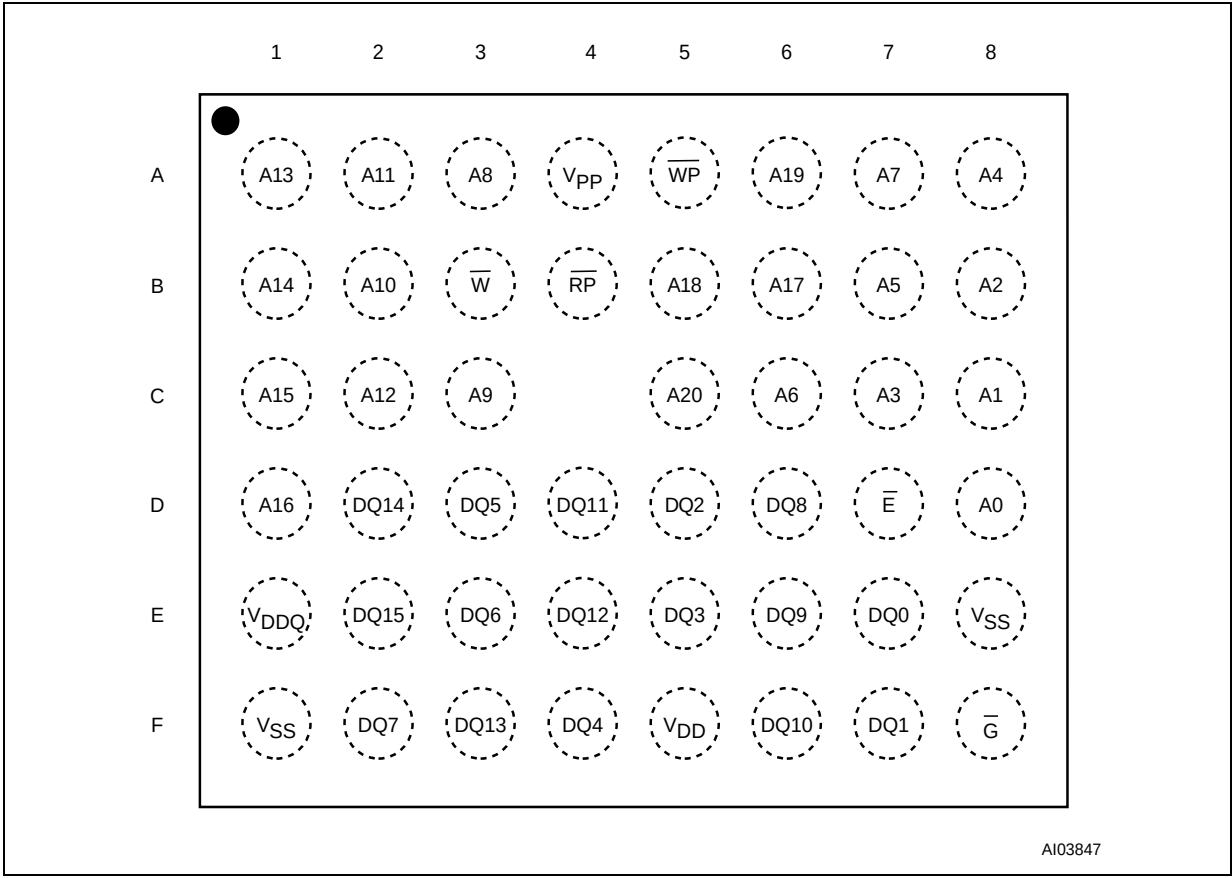
Figure 4. TFBGA Connections (Top view through package)
