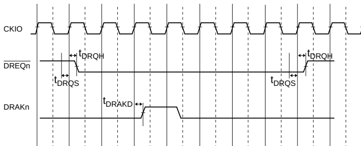
Figure 23.64(a) \overline{DREQ} /DRAK Timing
