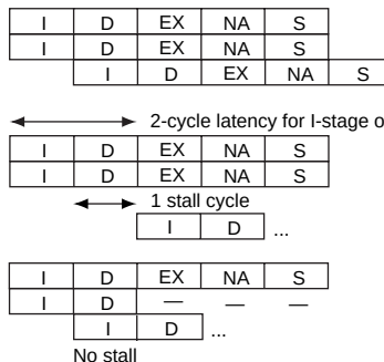
Figure 8.3 Examples of Pipelined Execution
