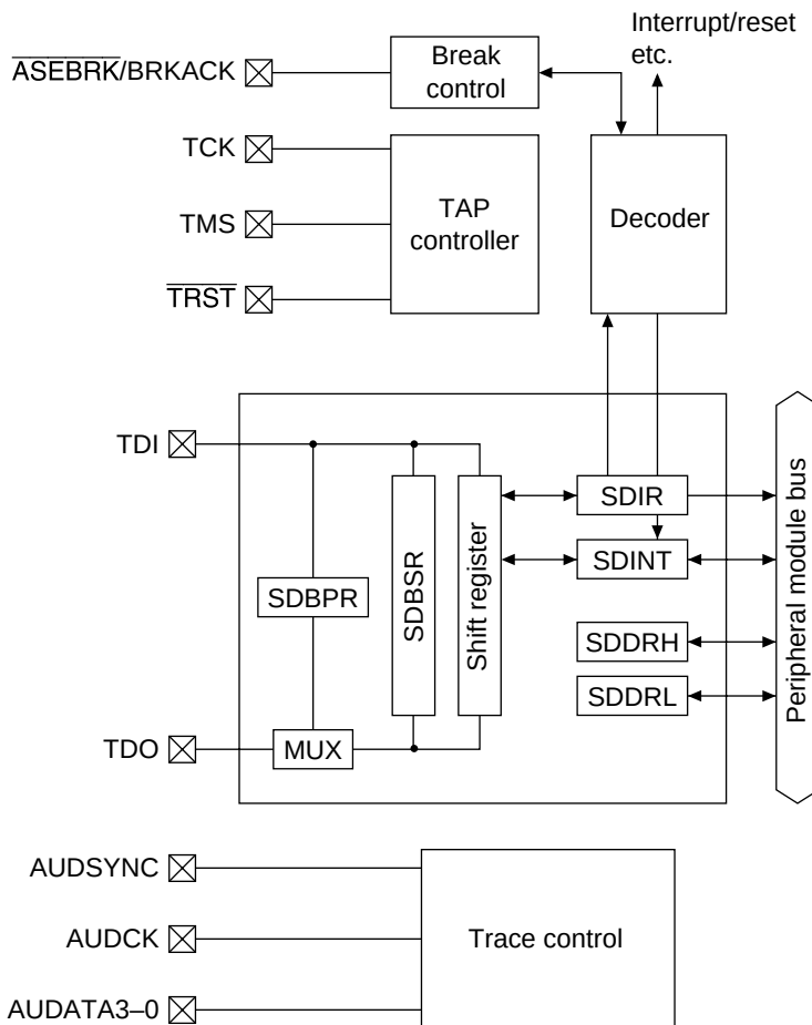
Figure 21.1 Block Diagram of H-UDI Circuit
