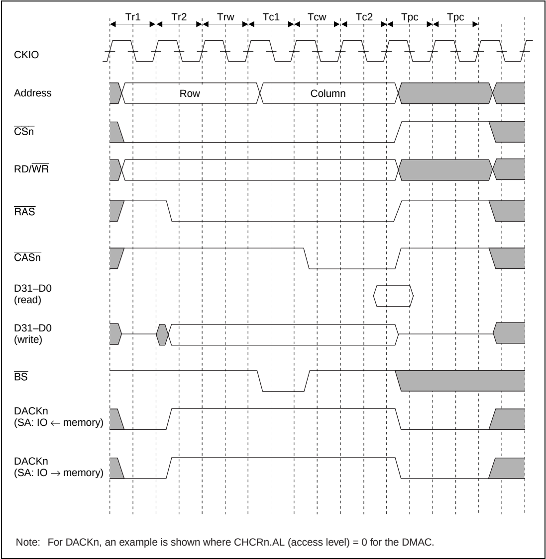
Figure 13.15 DRAM Wait State Timing
