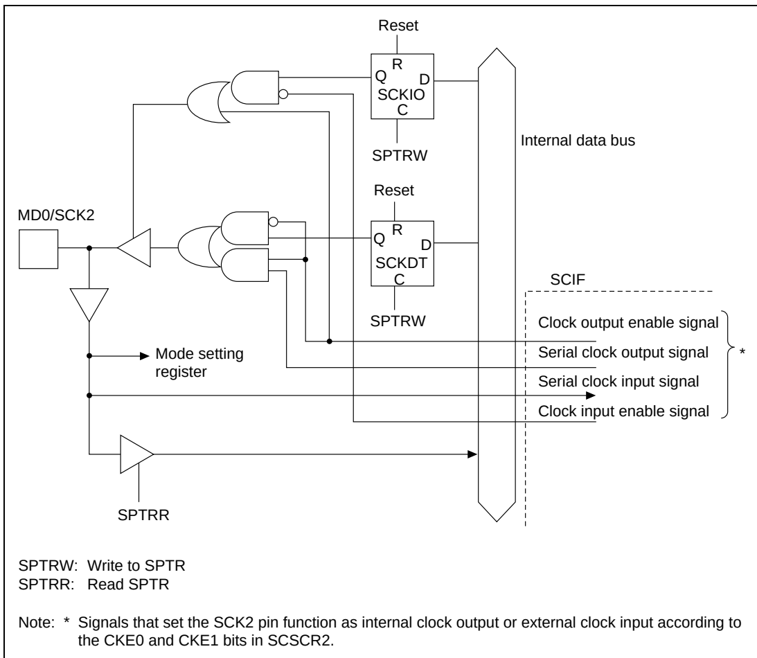
Figure 16.6 MD0/SCK2 Pin
