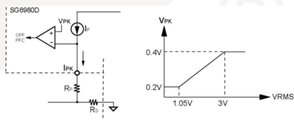
FIG.6 Current Limit
