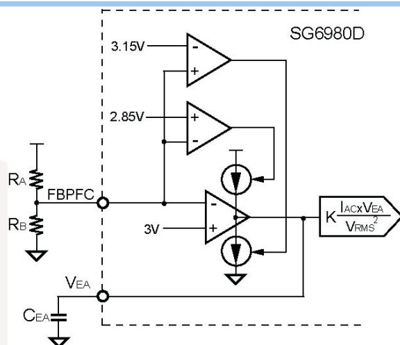
FIG. 5 Voltage Error Amplifier with Multi-Vector
