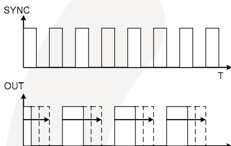
FIG.3 Synchronized Interleaving-Switching
