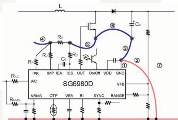
FIG. 7 PCB Layout
