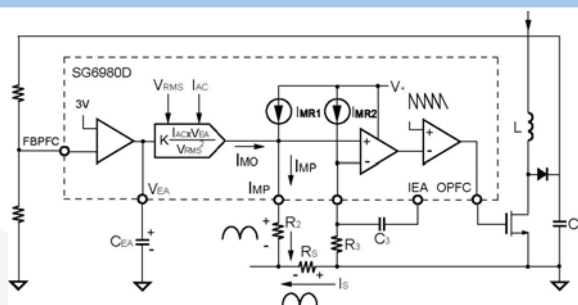
FIG.4 Multiplier and Control Loop of PFC Stage
