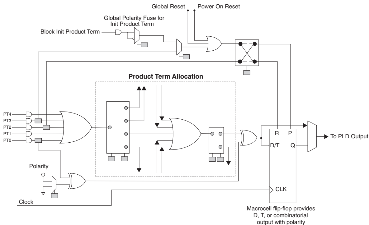
Figure 10. ispPAC-POWR1014/A Macrocell Block Diagram
