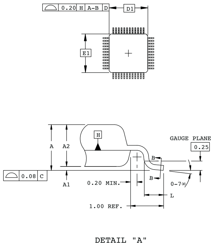
DETAIL "A"
