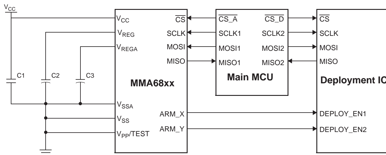
Figure 1. Application Diagram
