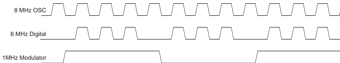
Figure 12. Clock Generation
