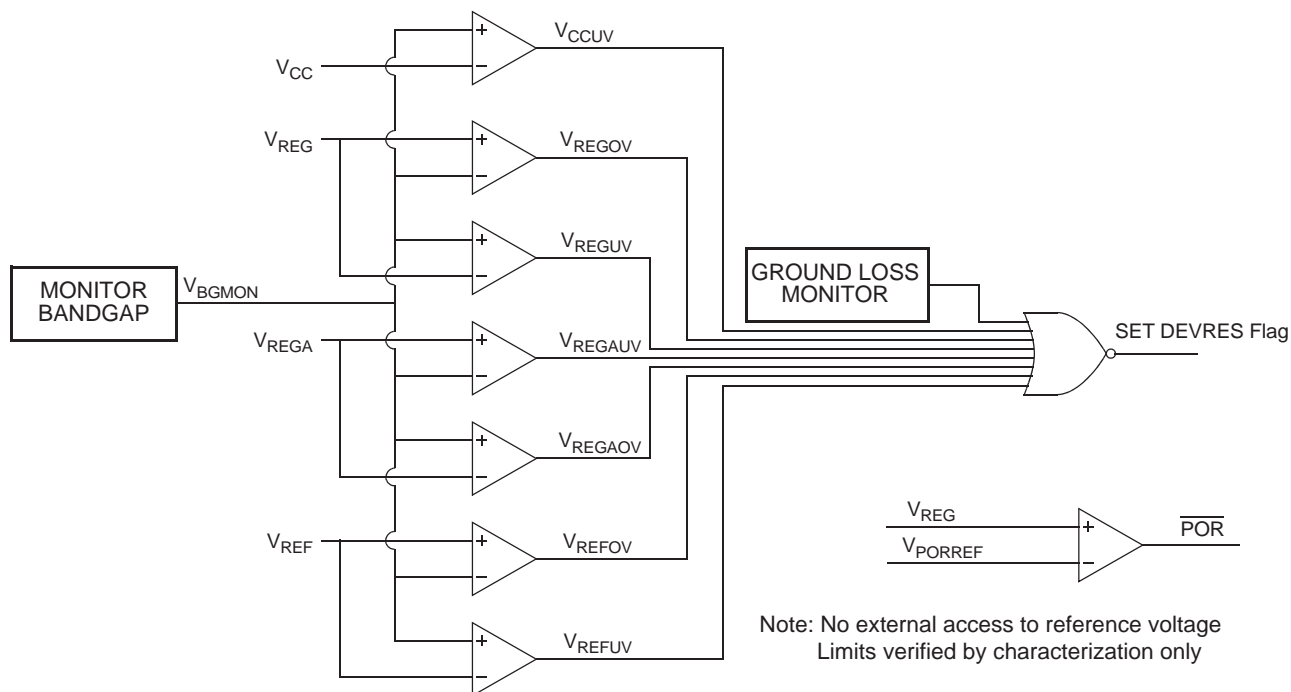
Figure 8. Voltage Monitoring
