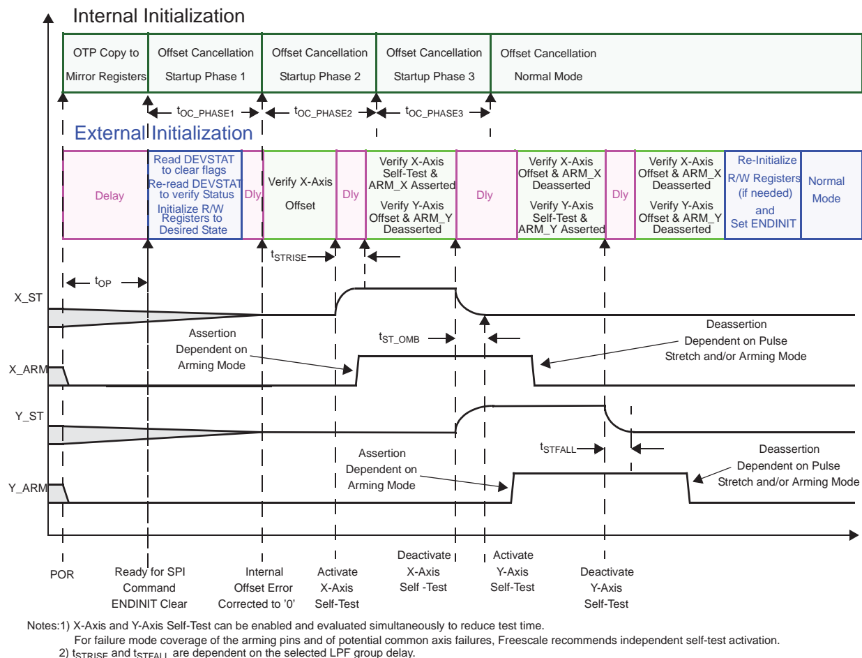
Figure 31. Initialization Process
