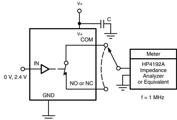
Fig. 7 - Source / Drain Capacitances
