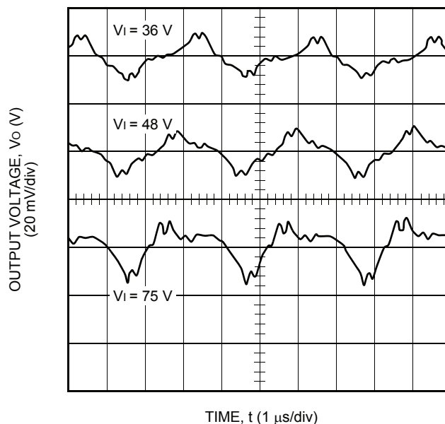
Figure 7. Typical JAHW050G Output Ripple Voltage at Room Temperature and I_o = I_{o, \max}
