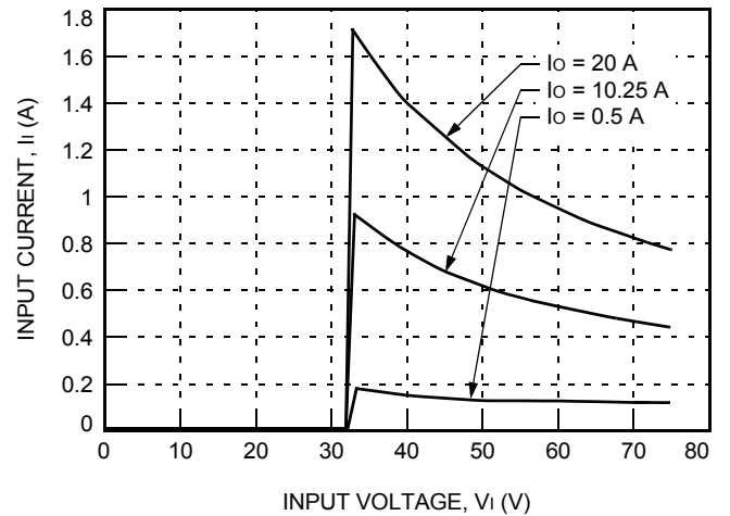
Figure 3. Typical JAHW100G Input Characteristics at Room Temperature
