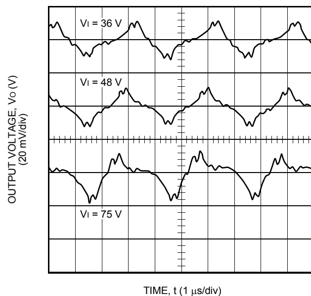
Figure 8. Typical JAHW075G Output Ripple Voltage at Room Temperature and I_o = I_{o, \max}
