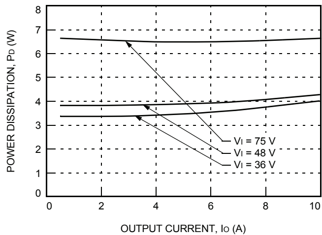
Figure 28. JAHW050G Power Dissipation vs. Output Current at 25 °C
