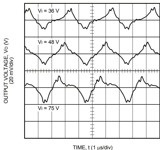
Figure 9. Typical JAHW100G Output Ripple Voltage at Room Temperature and I_o = I_{o, \max}
