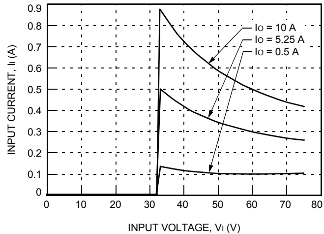
Figure 1. Typical JAHW050G Input Characteristics at Room Temperature
