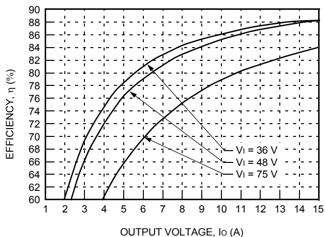
Figure 5. Typical JAHW075G Converter Efficiency vs. Output Current at Room Temperature
